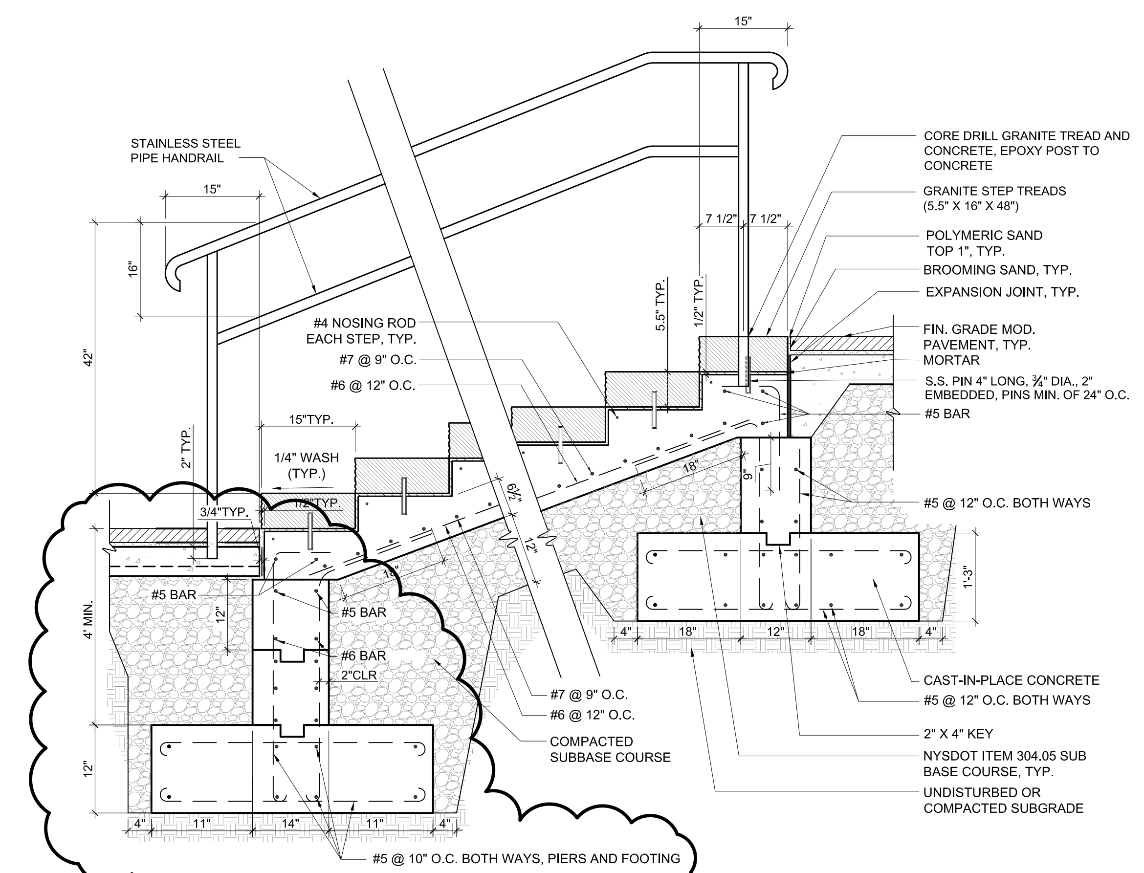
1 GRANITE STEPS ON CONCRETE BASE SKC-1 Scale: 3/4" = 1'-0"
