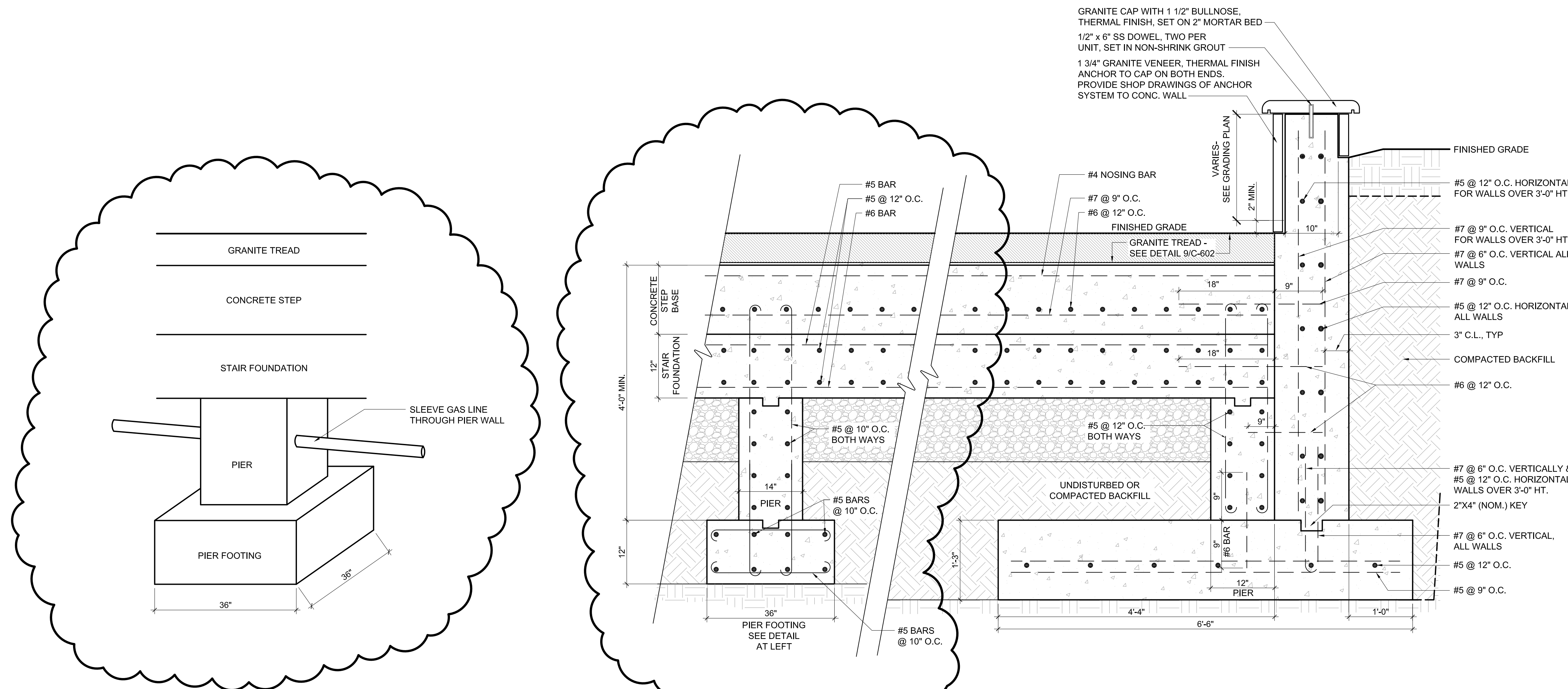
2 WALL B AND STAIR FOUNDATION
