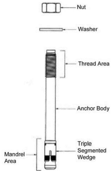
FIGURE 1—KWIK BOLT 3
