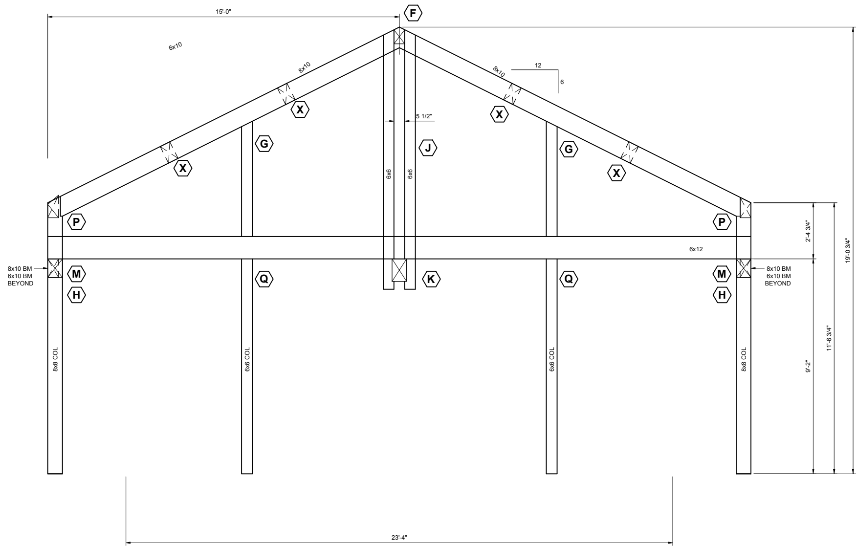
BENT #5 SCALE: 1/2"=1'-0" REFER TO DWG S01 FOR DRAWING NOTES
