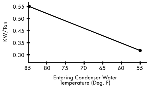
Fig. 6: Algorithm: kW/ton = 0.34 + (0.007 \times [EWT-55])
