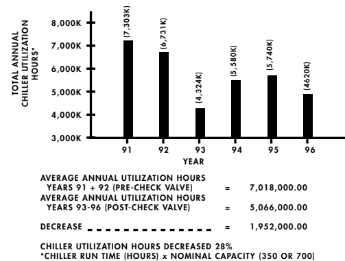
Fig. 3: Annual chiller utilization.
