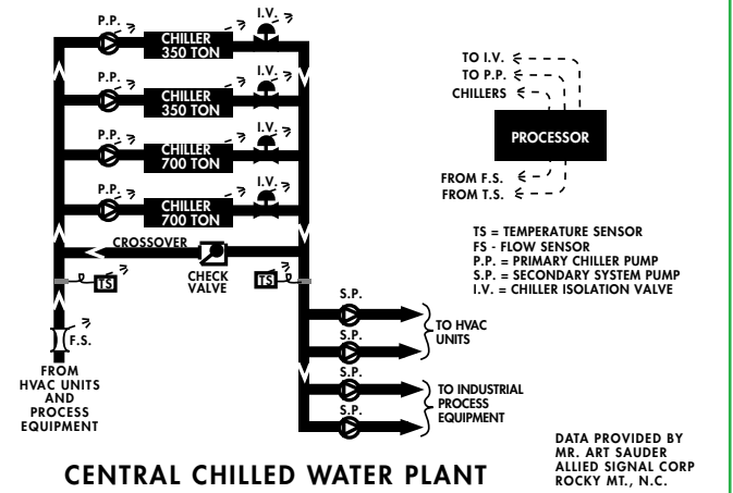
Fig. 1: Central chilled water plant
