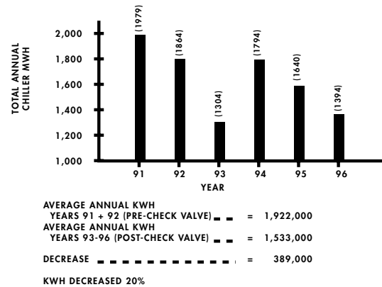
Fig. 2: Annual chiller MWH.
