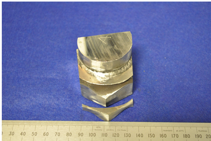
Cross sectional view of bolts failure
