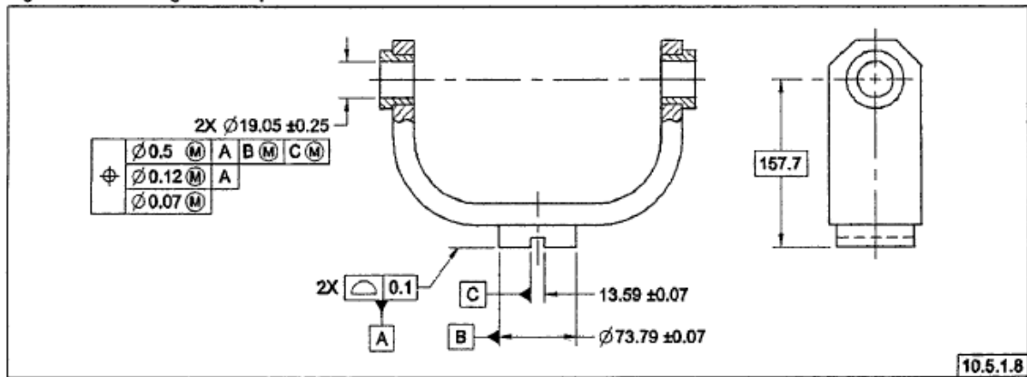
Fig. 10-46 Three Segment Composite Tolerance
