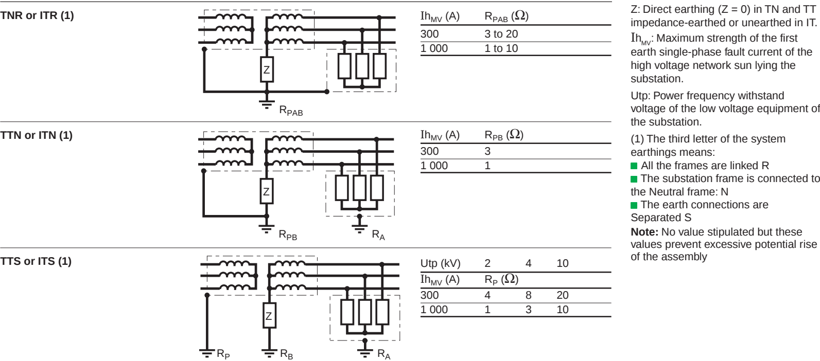
Fig. 19 : Maximum resistance of the earth connection of the substation frames according to network system earthing (used in France)
