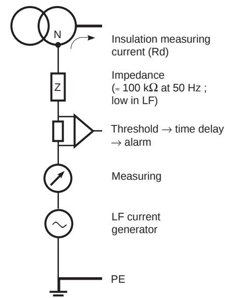
Fig. 25 : Functional diagram of an Insulation Monitoring Device (IMD)
