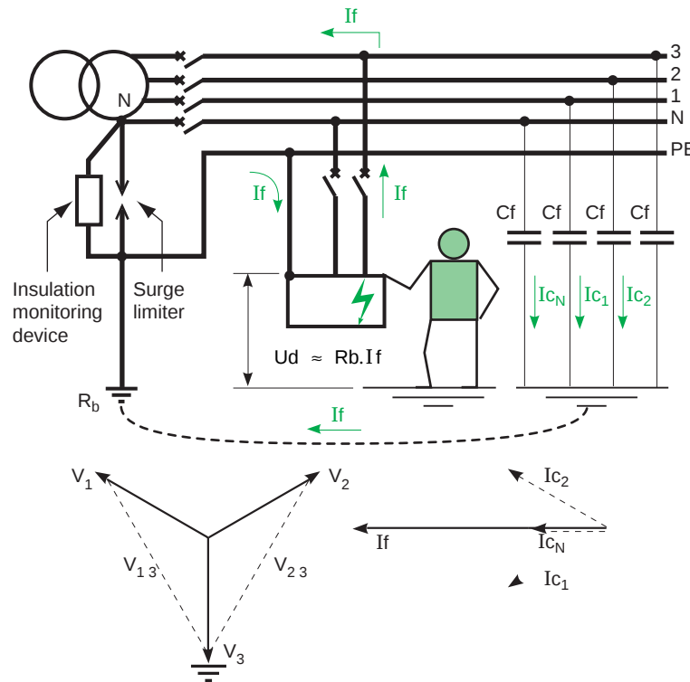
Fig. 12 : First insulation fault current in IT system
