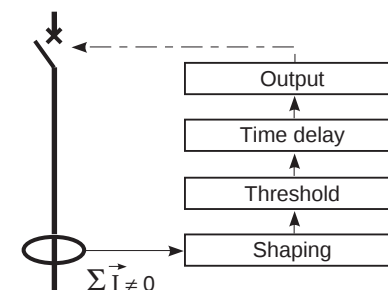
Fig. 24 : Functional diagram of an RCD
