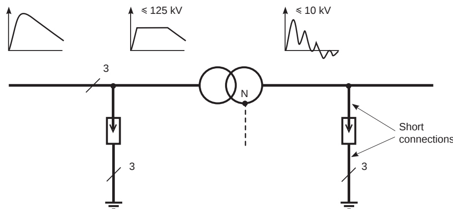
Fig. 18 : Limitation and transmission of lightning overvoltages (whether or not the neutral is earthed, there are common mode overvoltages on phases)
