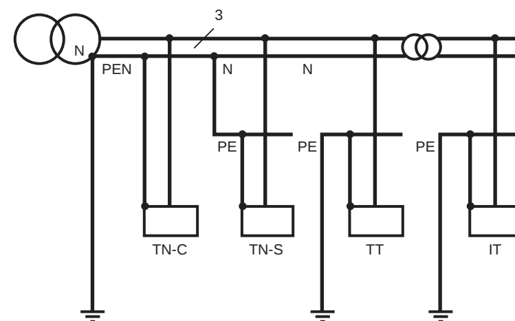
Fig. 6 : Example of the various system earthings included in the same installation
