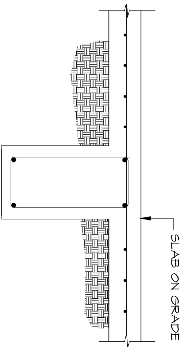
CONTRACTOR'S DETAIL
