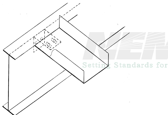
Figure 4.50 TRAY TO CHANNEL
