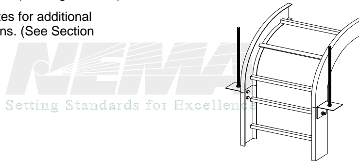
Figure 4.18 VERTICAL SUPPORT PLATES
