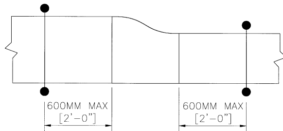
Figure 4.25 HORIZONTAL CROSS
