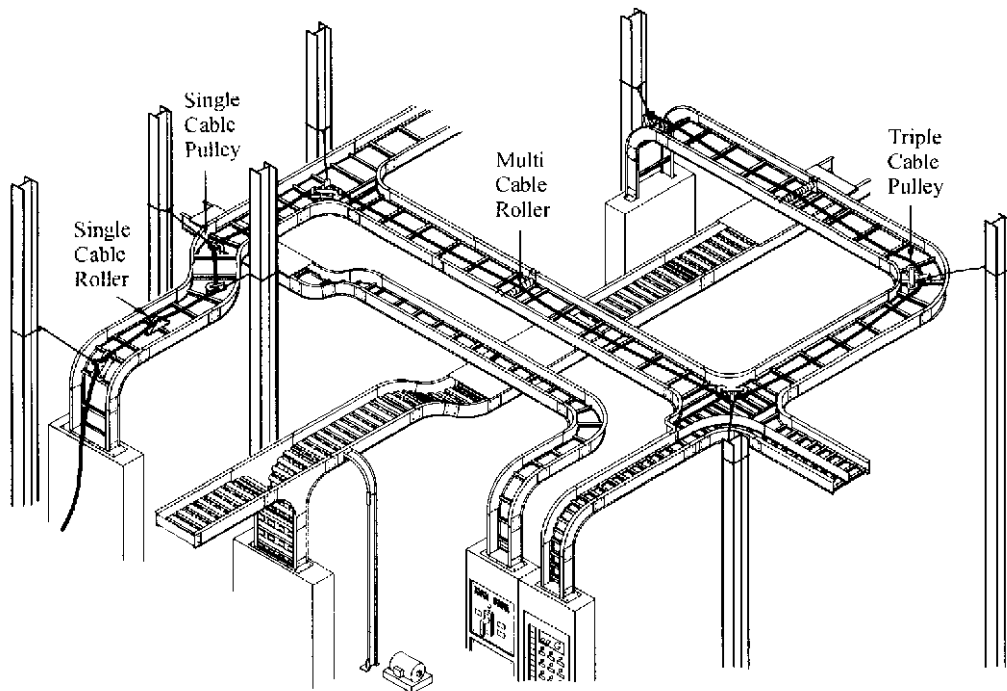
Figure 5.1 CABLE INSTALLATION
