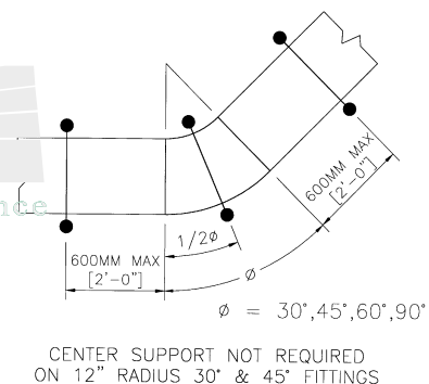
Figure 4.22 HORIZONTAL ELBOWS
