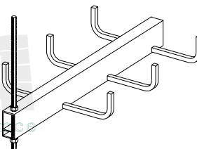
Figure 4.6B ROD THROUGH SPINE HANGER
