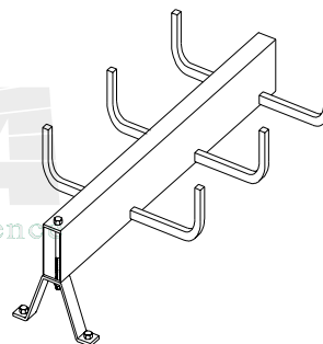
Figure 4.8C SINGLE RAIL FLOOR SUPPORT
