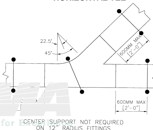
Figure 4.23 HORIZONTAL TEE
