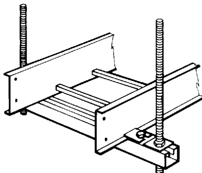
Figure 4.1C STRUT SUPPORT
