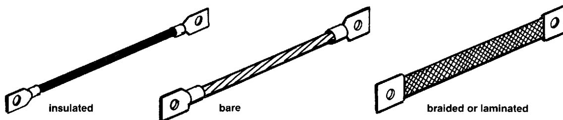
Figure 4.62 BONDING JUMPERS
