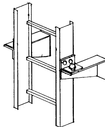
Figure 4.9B VERTICAL GUSSET CANTILEVER SUPPORT
