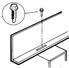
Figure 4.43 BARRIER STRIP ATTACHMENT, SELF-DRILLING AND SELF-TAPPING SCREW
