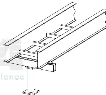
Figure 4.8A ELEVATED STRUT TYPE SUPPORT
