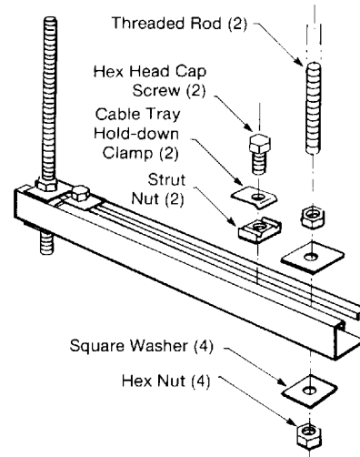
Figure 4.1F STRUT-EXPLODED VIEW
