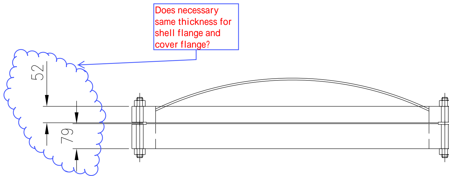
COVER FLANGE WITH SPHERE PLATE
