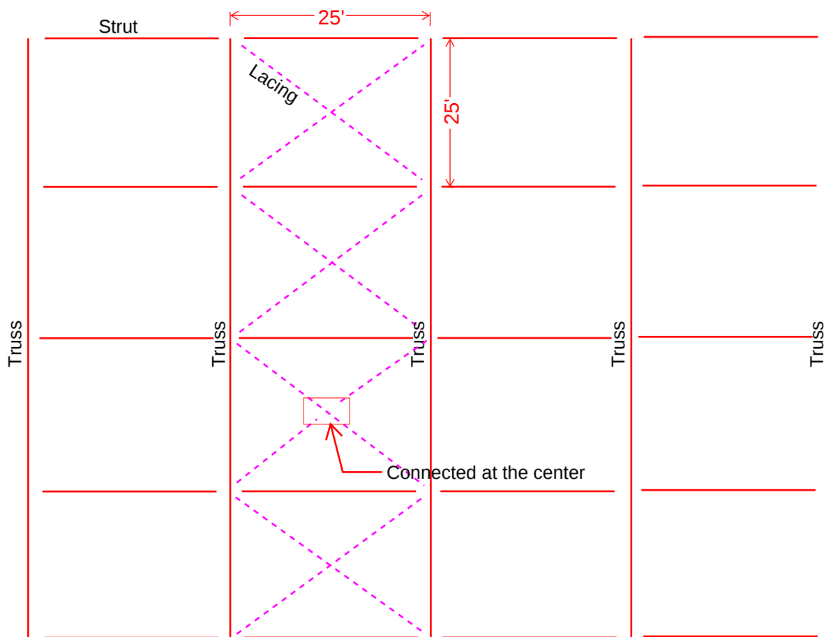
Plan View
