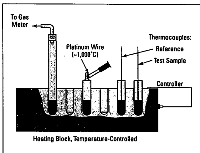
■ Figure 3. Luteflo oven evaluates exothermic-reaction temperatures for materials exposed to heat for long periods at lean oxygen concentrations.
