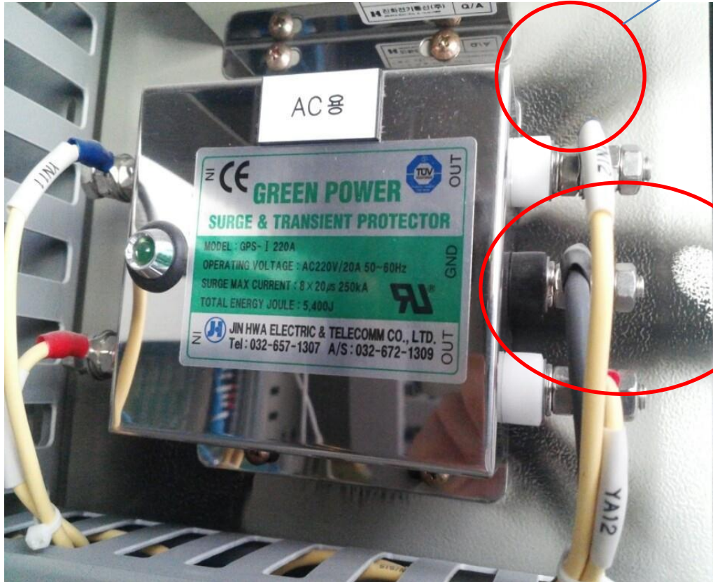
Damaged Surge Protector in AC Power Panel
