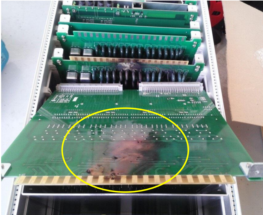
Damaged DO boards of Transformer Protection IED
