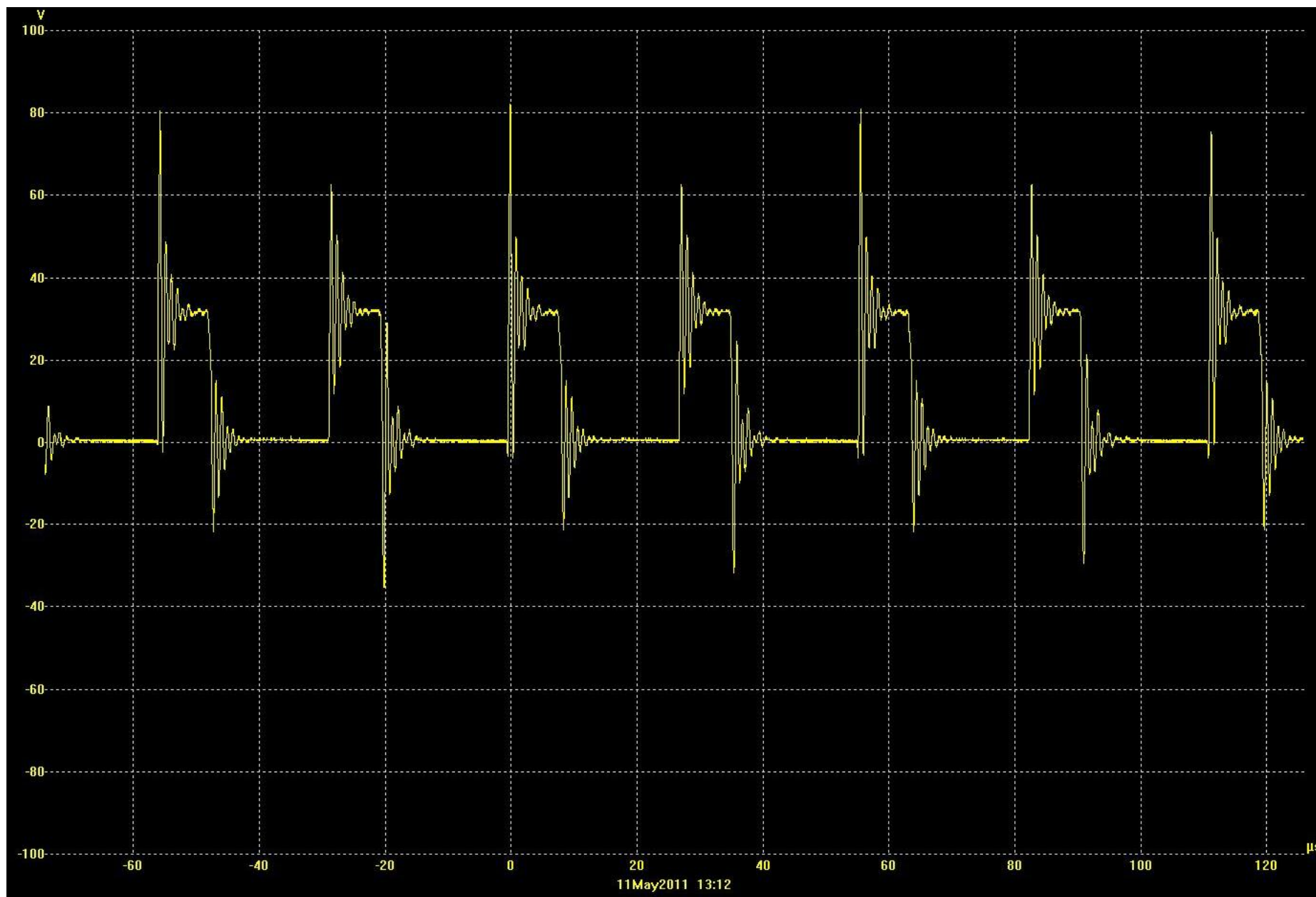
Motor 7 terminal box, zoom (about 800V ringing)
