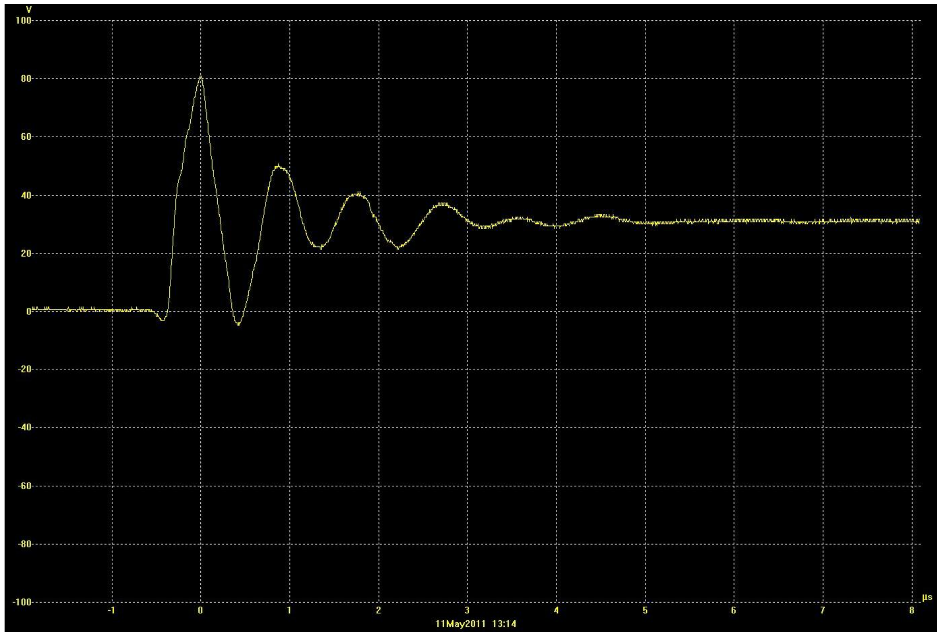
Motor 7 terminal box, zoom (about 800V, 1MHz ringing)
