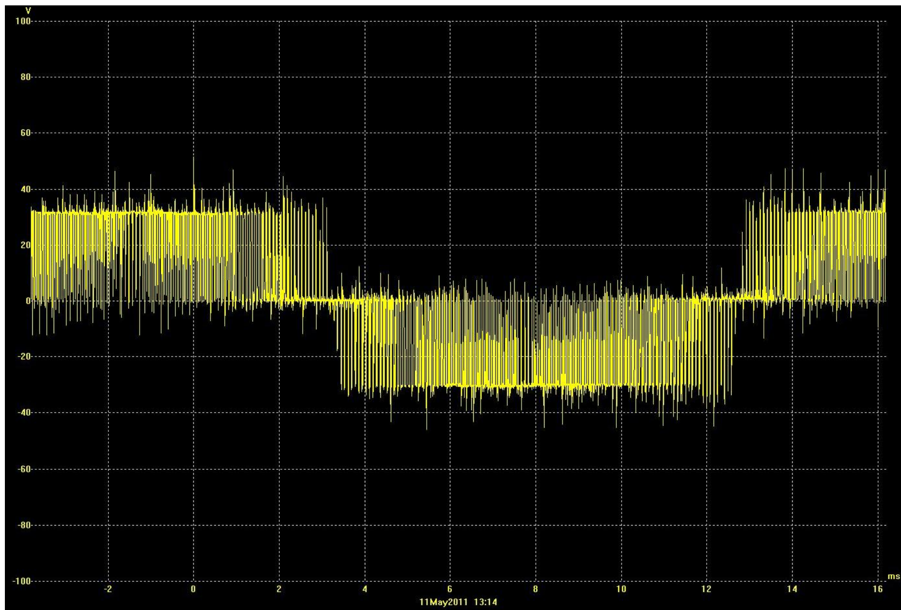
Motor 7 terminal box (here seen about 550V)
