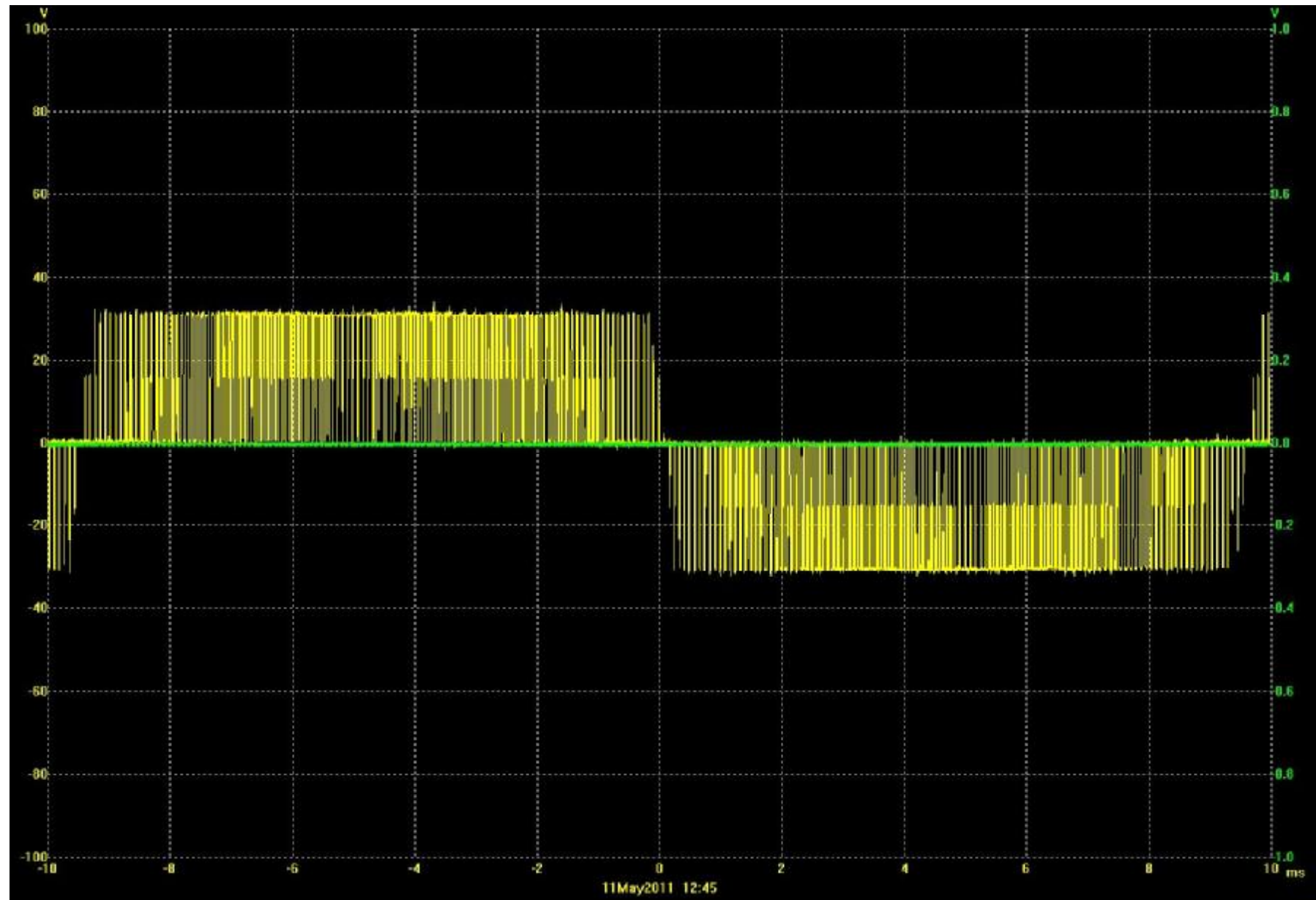
VFD output (310V peak, vertical scale 1:10)
