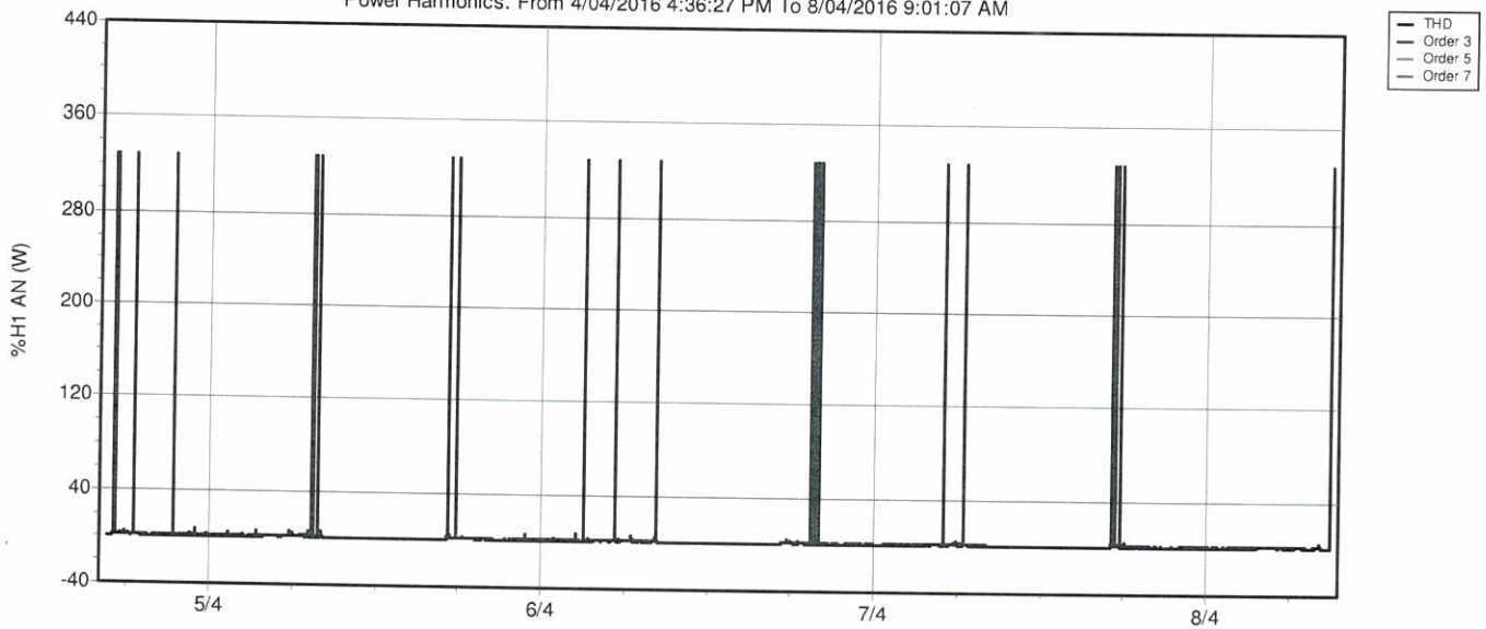
Power Harmonics. From 4/04/2016 4:36:27 PM To 8/04/2016 9:01:07 AM
