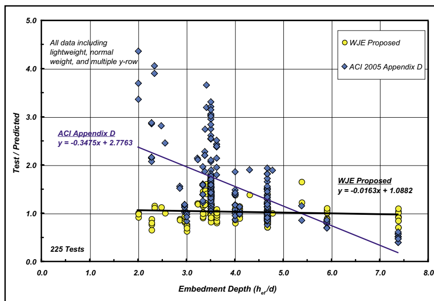
Fig. 23. Test-to-predicted capacity versus embedment depth ratio ( h_{ef}/d ) for all test data comparing the average equations from ACI 318-05 Appendix D and the proposed Eq. (5).
