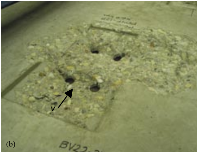
Fig. 11. Failure conditions of Test PO4F-12B with y = 6 in. (152 mm): (a) Deformation of studs after test; (b) Perspective view of the concrete breakout on the slab.
