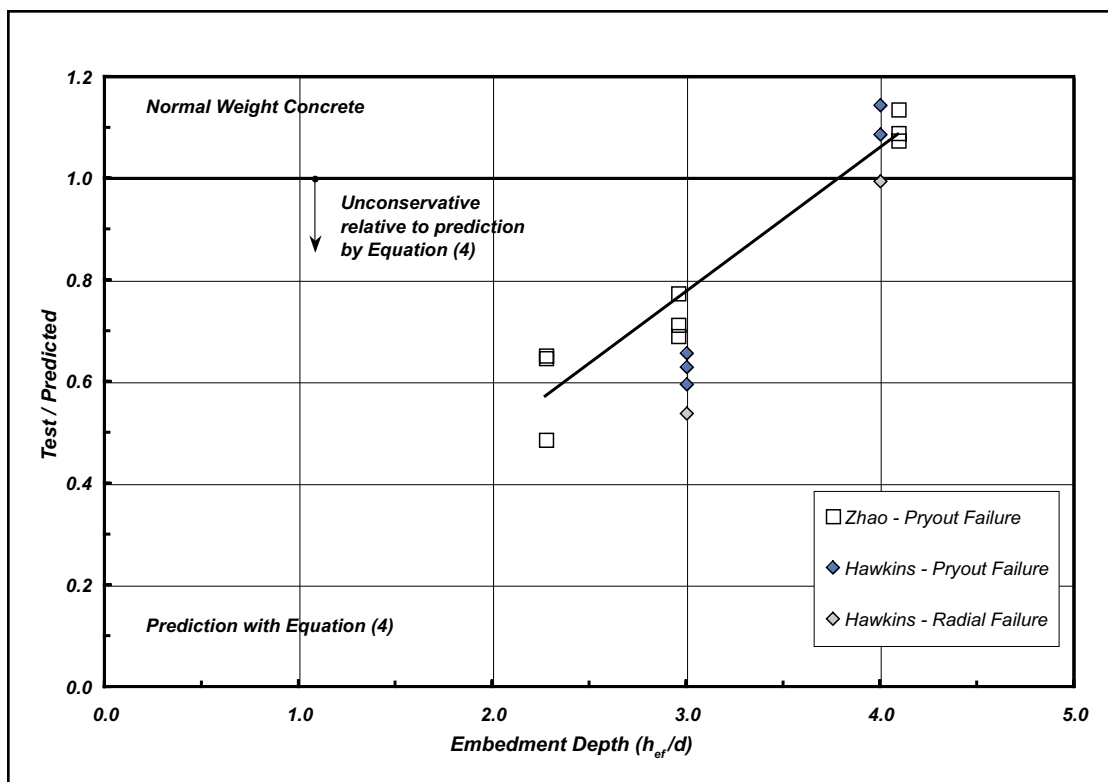
Fig. 5. Test-to-predicted capacity versus embedment depth using Eq. (4) for the Hawkins 9 and Zhao 10 pryout test data.
