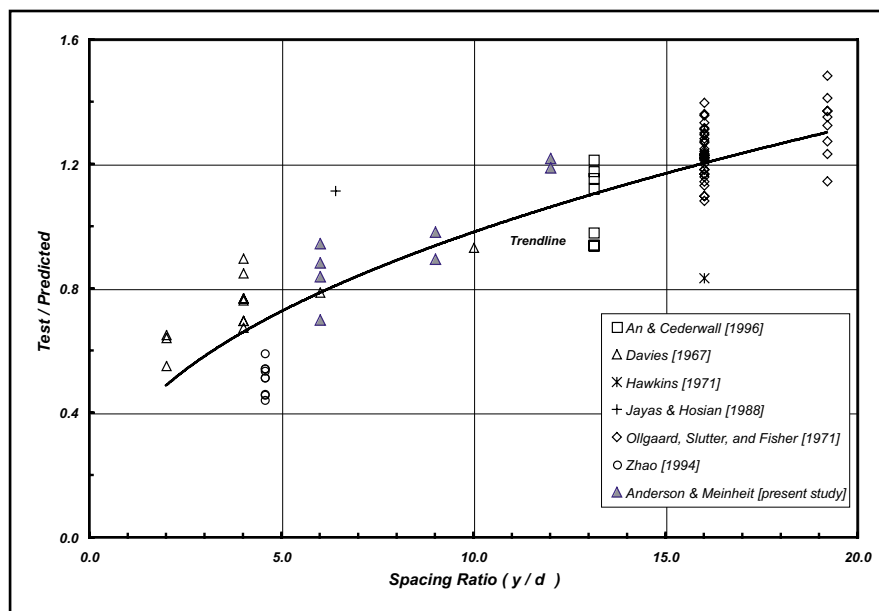
Fig. 19. Test-to-predicted capacity using Eq. (5) versus spacing ratio ( y/d ) for the multiple y -row pushoff and pryout tests.
