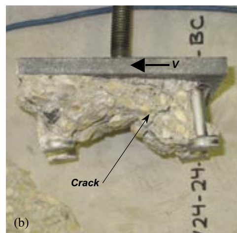
Fig. 10. Failure conditions of Test PO4F-9A and -9B with \gamma = 4.5 in. (114 mm): (a) Concrete breakout plan of both tests on slab; (b) Connection plate with concrete intact with crack propagating from front studs to rear.
