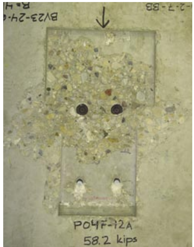
Fig. 12. Mixed mode failure of Test PO4F-12A with y = 6 in. (152 mm) showing steel failure of front studs and concrete breakout at the rear studs.
