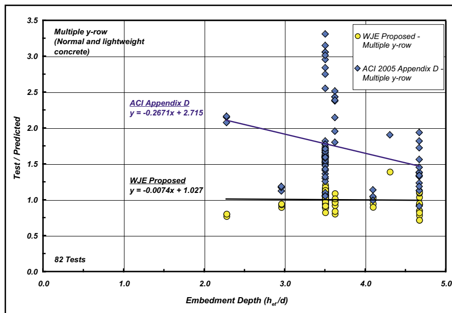
Fig. 22. Test-to-predicted capacity versus embedment depth ratio ( h_{ef}/d ) for multiple y-row tests comparing the average equations from ACI 318-05 Appendix D and the proposed Eq. (5).
