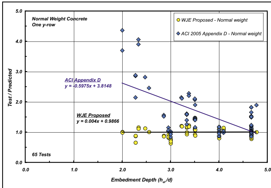
Fig. 20. Test-to-predicted capacity versus embedment depth ratio ( h_{ef}/d ) for normal weight concrete, one y-row tests comparing the average equations from ACI 318-05 Appendix D and the proposed Eq. (5).
