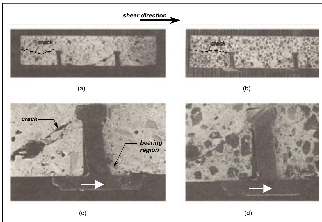
Fig. 15. Splitting cracks in (a) and (b) observed in the rear stud of the pushoff test specimens (from Ollgaard et al. 5 ): (a) Normal weight concrete (Specimen LA1); (b) Lightweight concrete (Specimen LE2); (c) Detail of front stud (Specimen LA1); (d) Detail of front stud (Specimen LE2). Note: Splitting cracks in (a) and (b) traced for reproduction purposes.
