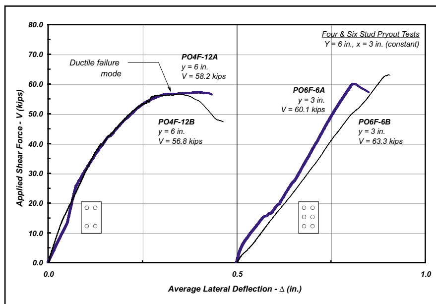
Fig. 18. Load-deflection curves for the four- and six-stud pryout tests with Y = 6 in. (152 mm).
