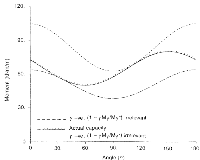
Fig 4(c). Solutions for \gamma from eqn. (9) with a negative applied field of moment
