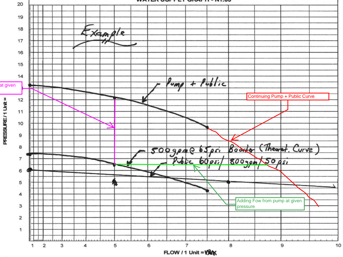
WATER SUPPLY GRAPH - N1.85
