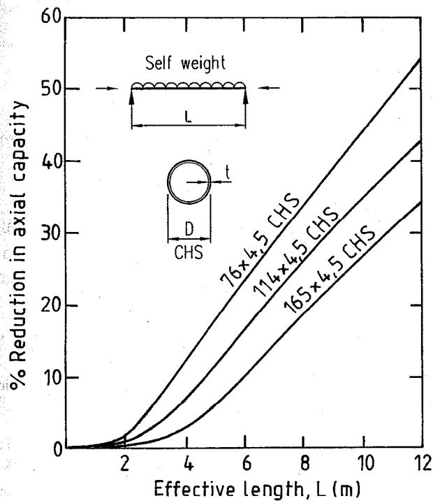
Figure 6.10 Reduction in Axial Capacity of CHS (Grade 250) Tubular Struts Due to Self Weight
