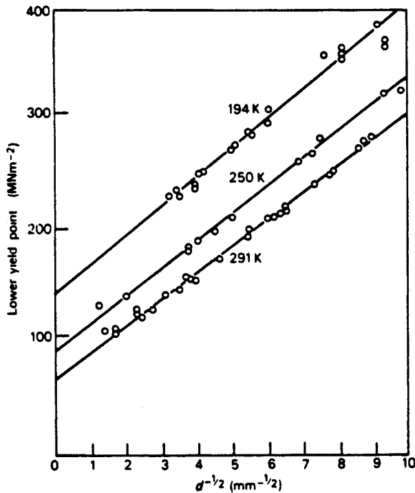
Figure 1. Dependence of the lower yield stress of mild steel on grain size.
