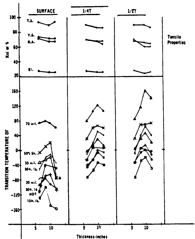
Figure 4. Surface to center variation of tensile and impact properties in 5 to 10 inch sections.
