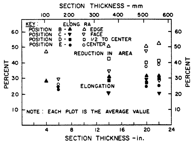
Fig. 15-72 Elongation and reduction in area as a function of section size and location within the annealed pivot arm of carbon steel in Figure 15-71 (1).
