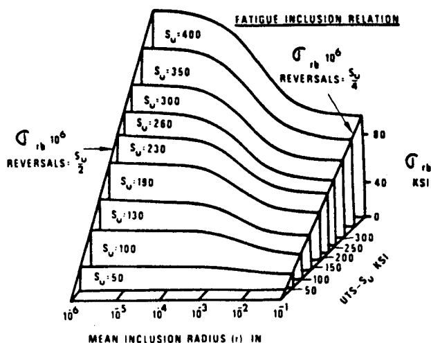
Figure 7. Effect of inclusion size on fatigue ( \sigma_{fb} ) as a function of ultimate tensile strength ( S_u ).
