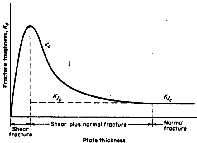
Figure 9. Schematic variation of the fracture toughness as a function of the plate thickness.
