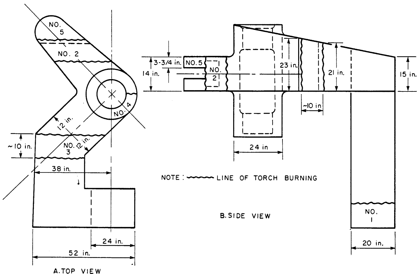
Fig. 15-71 A. Top view of pivot arm with significant dimensions. B. Side view of pivot arm with significant dimensions. Conversion: 1 in. = 25.4 mm.
