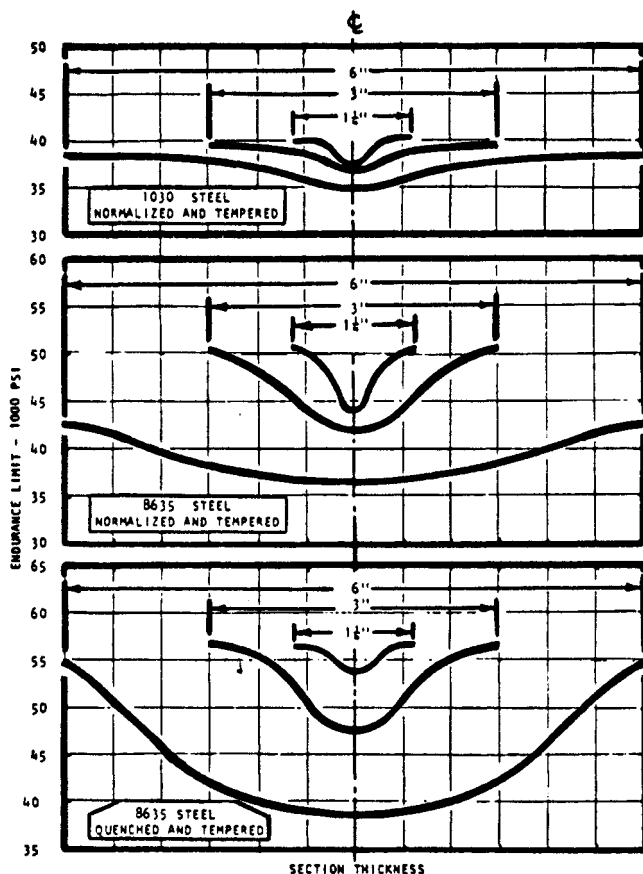
Figure 5. Distribution of endurance limit across the thickness of steel castings of several section thicknesses.
