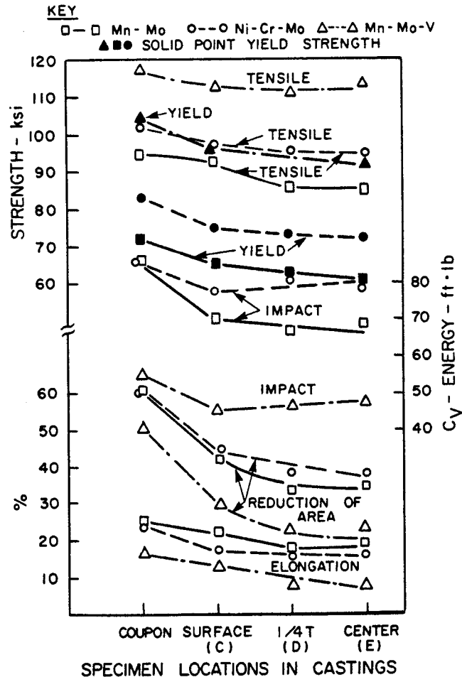
Fig. 15-69 Mechanical properties of specimens cut from various locations of quenched and tempered low alloy steel production castings (Compositions given in Table 15-22) (1). Conversion: 1 ksi = 6.895 MPa, 1 ft-lb = 1.356 J.
