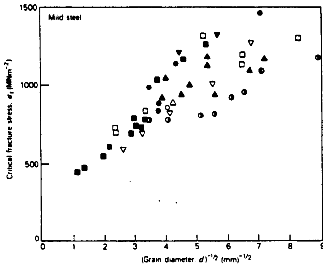
Figure 2. Dependence of local fracture stress of on the grain size of mild steel.
