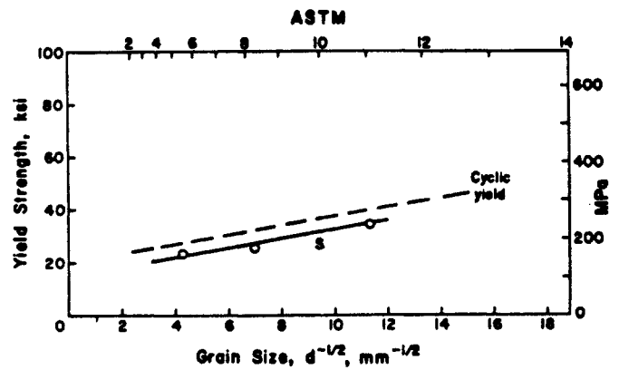
Figure 3. Effect of grain size on endurance limit of a low-carbon steel.
