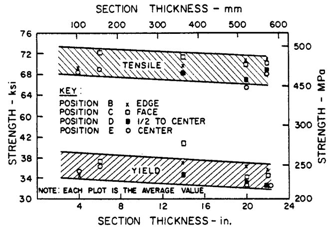
Fig. 15-70 Tensile and yield strength as a function of section size and location within the annealed pivot arm of carbon steel in Figure 15-71 (1).
