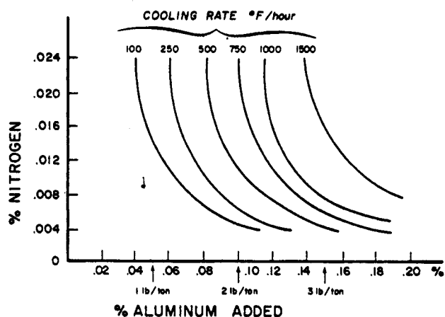
Figure 8. A chart to indicate approximate limits of nitrogen and aluminum that may be tolerated in a base analysis containing 0.30% C, 1.60% Mn, 0.50% Si, 0.50% Cr, and 0.35% Mo without development of intergranular type fracture.
