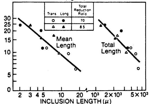
Figure 6. Effect of inclusion length on absorbed energy in the longitudinal and transverse direction.
