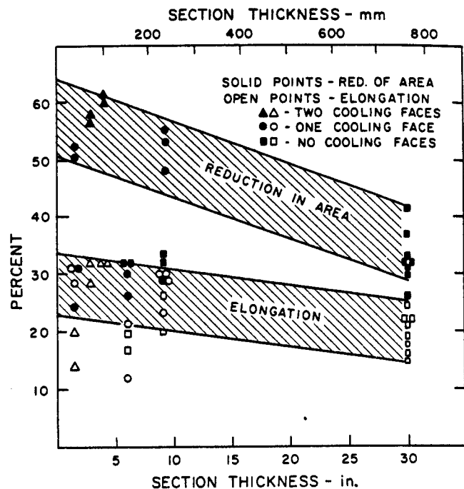
Fig. 15-75 Effect of section size on tensile ductility, at 1/4 T and center locations, of a normalized and tempered turbine blade casting of Ni steel (0.2%C, 2.4%Ni) (1).
