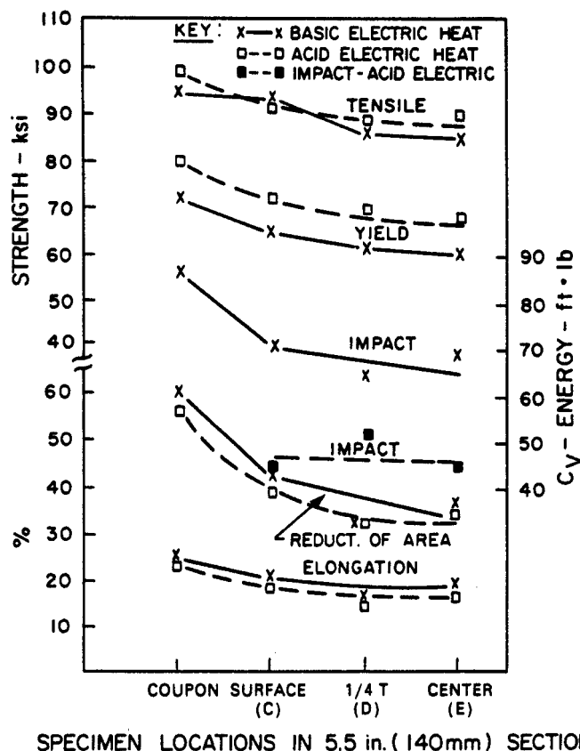
Fig. 15-68 Mechanical properties of specimens cut from various locations of two quenched and tempered Mn-Mo production castings (Composition in Table 15-22) (1). Conversion: 1 ksi = 6.895 MPa, 1 ft·lb = 1.356 J.
