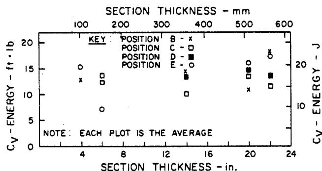
Fig. 15-73 Room temperature Charpy V-notch impact properties as a function of section size and location within the annealed pivot arm of carbon steel in Figure 15-71 (1).
