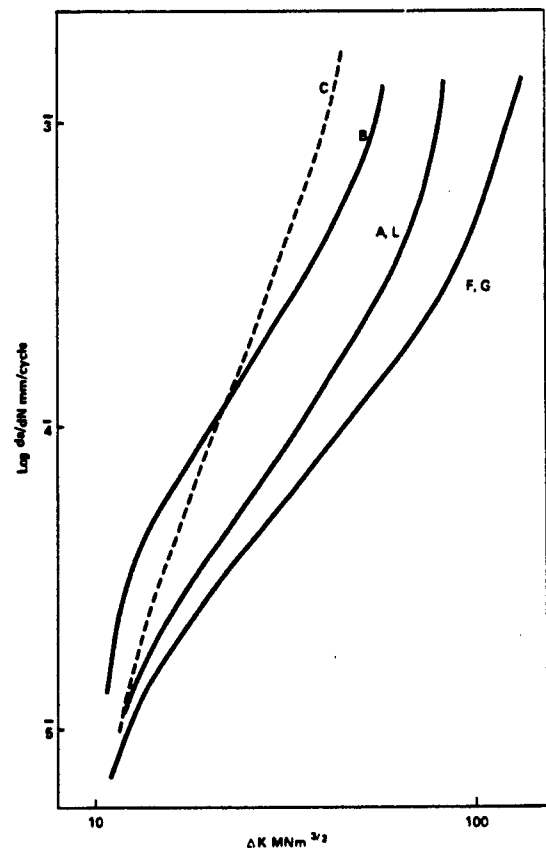
Figure 10. Fatigue crack propagation curves for six steels (A = 1 1/2% Mn, B = 1/2% Cr - 1/2% Mo - 1/4% V, C = 1 1/2% Mn - 3/4% Ni - 1/2% Cr-Mo, F = 1 1/2% Mn-Mo, G = 1 1/2% Ni-Cr-Mo, L = 0.54% C).
