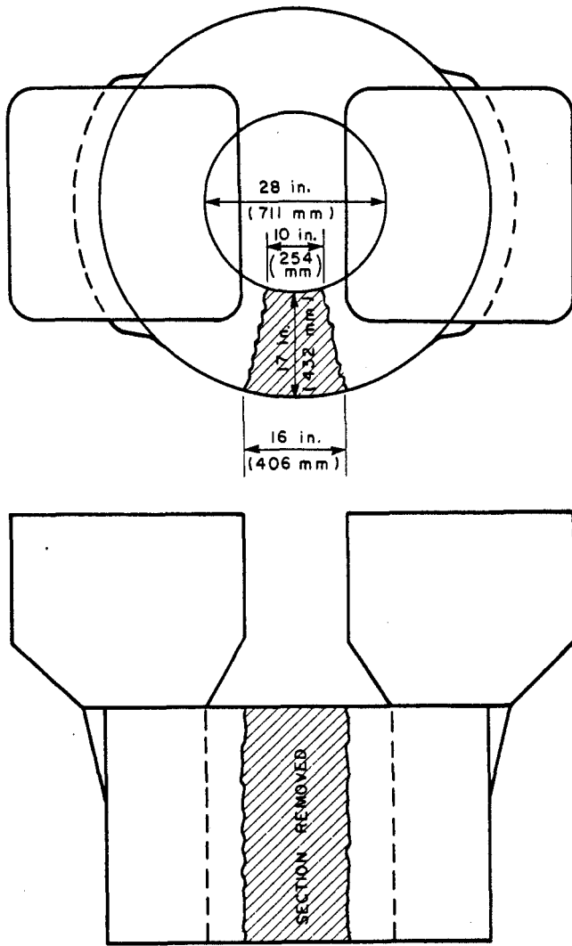
Fig. 15-76 Sketch of cast gear, quenched and tempered cast 8630 steel, showing location of section from which trepanned specimens were removed.
