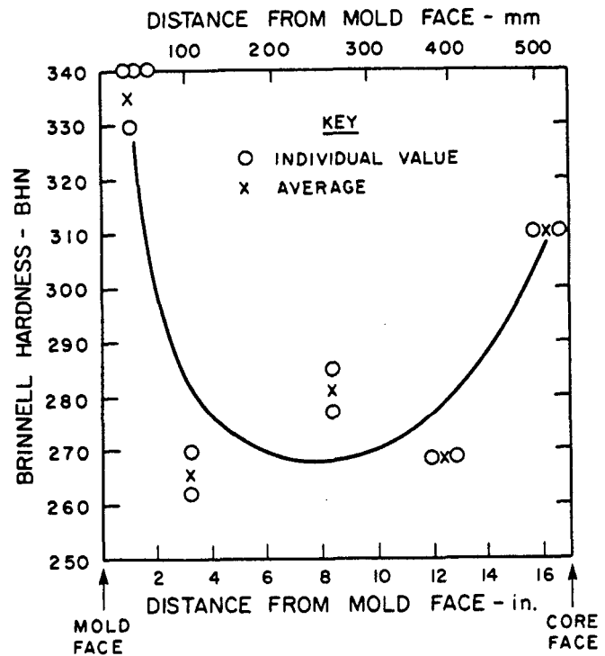
Fig. 15-77 Effect of distance from cooling faces (mold and core) on hardness of a gear blank face shown in Figure 15-76 (1).
