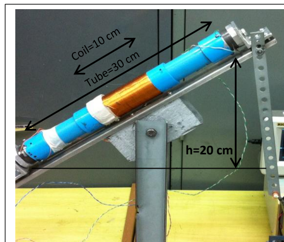
Test system
