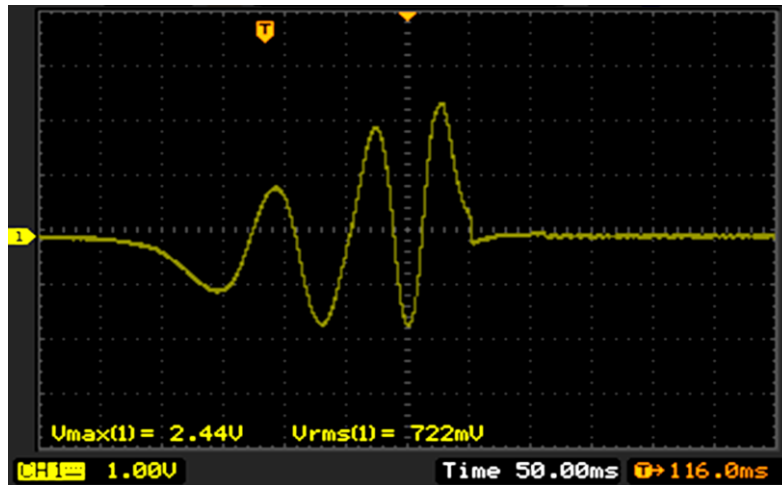
Output waveform form the coil
