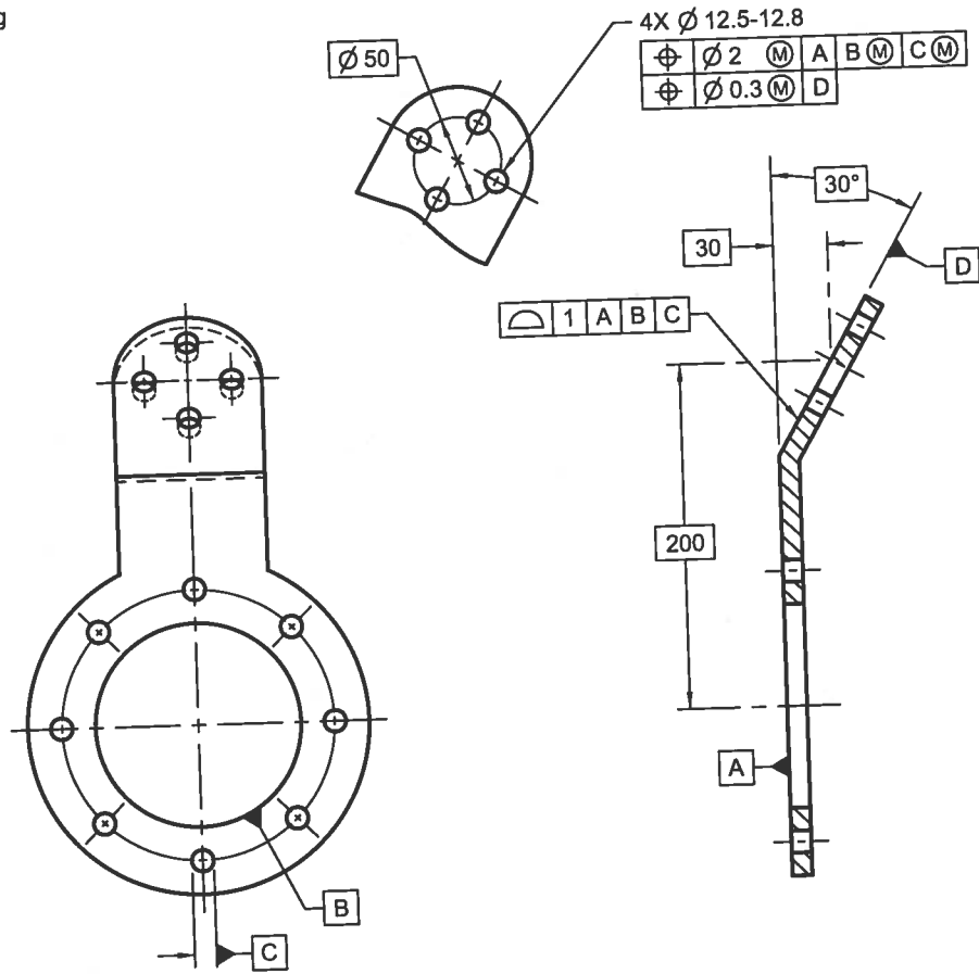
Fig. 7-55 Multiple Positional Tolerancing for a Pattern of Features
