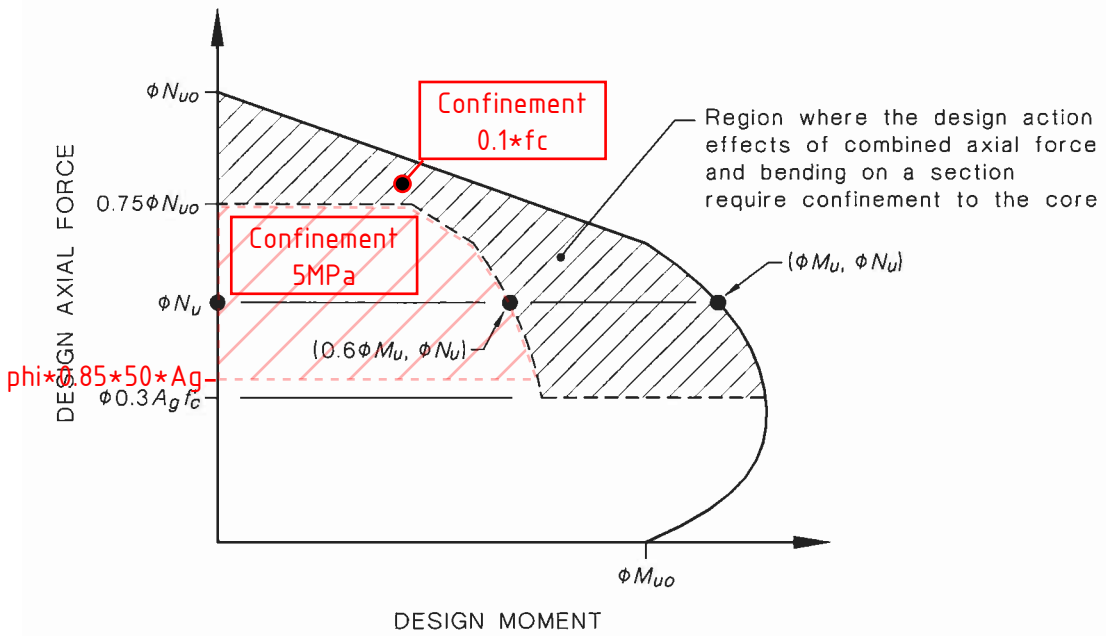
FIGURE 10.7.3.1(A) CONFINEMENT TO THE CORE
