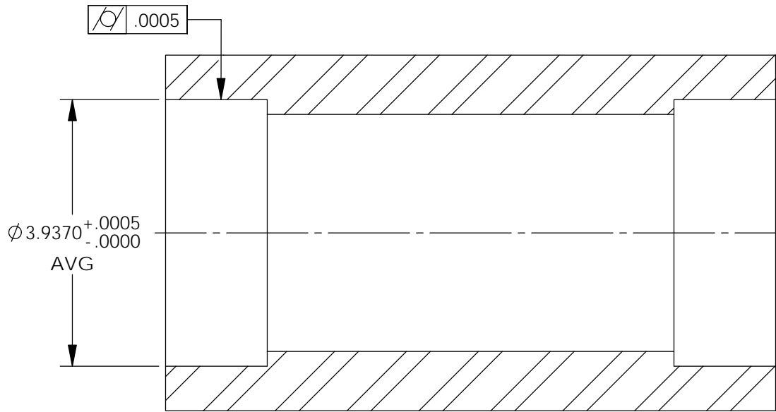
SECTION B-B HOUSING
