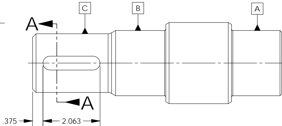
SHAFT
