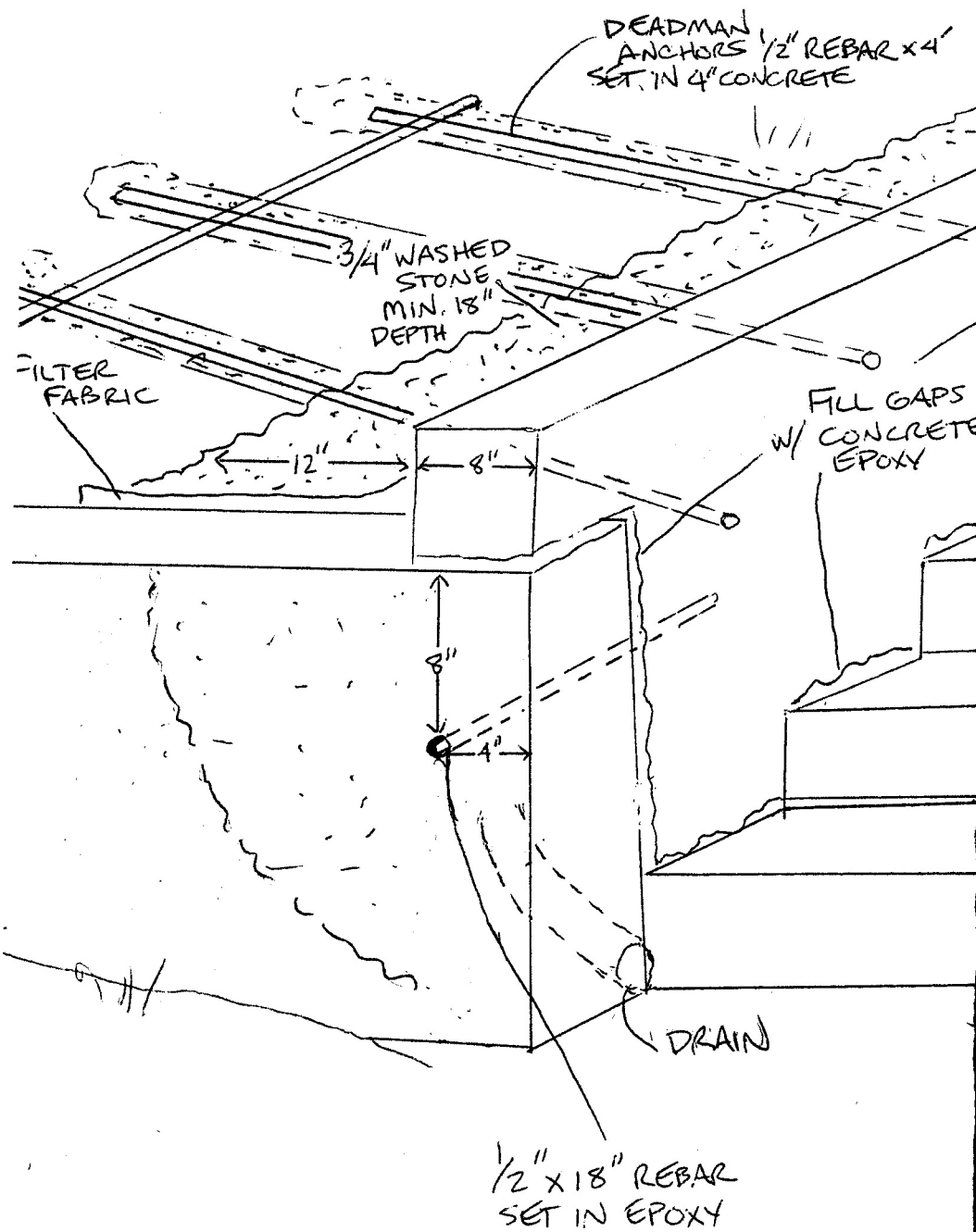
EXISTING CONCRETE RETAINING WALL REPAIR
