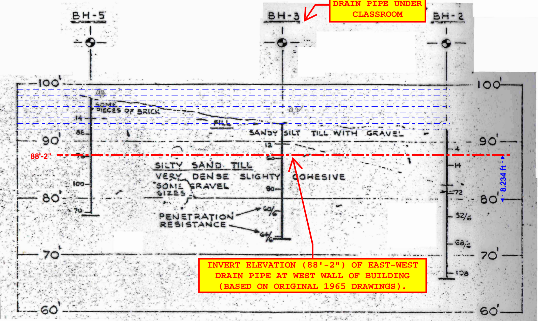
INTERPRETED SUBSOIL STRATIGRAPHY. SCALE: HOR. 1" = 30'-0" VERT. 1" = 10'-0"
