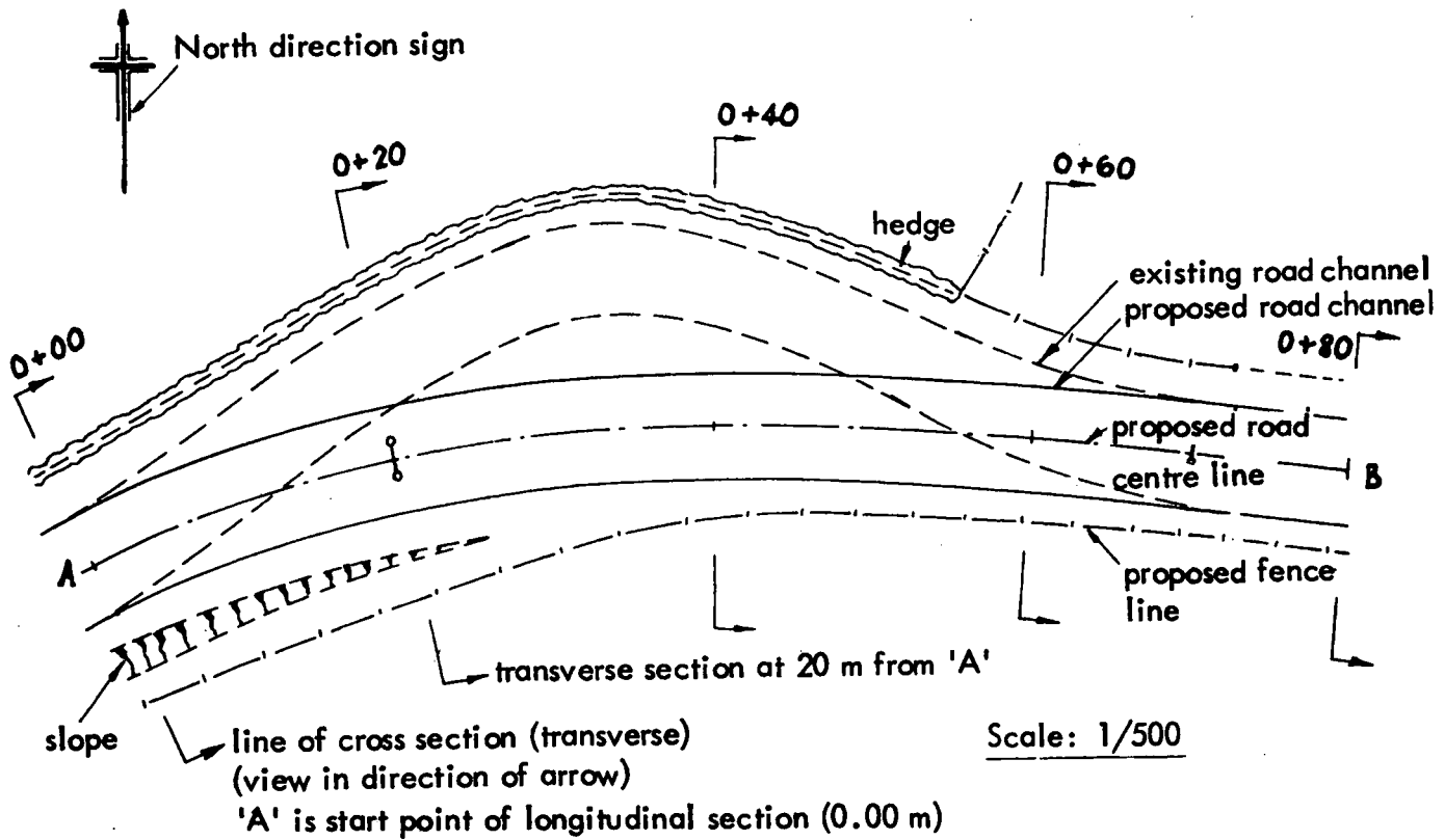
Figure 2.1 Example of a Highway Survey Plan. Note that chainages may start at 100 m to avoid the possibility of negative chainage values. Also, in order to be computer compatible, chainages may be shown as 000, 020, rather than 0+00, 0+20, etc.
