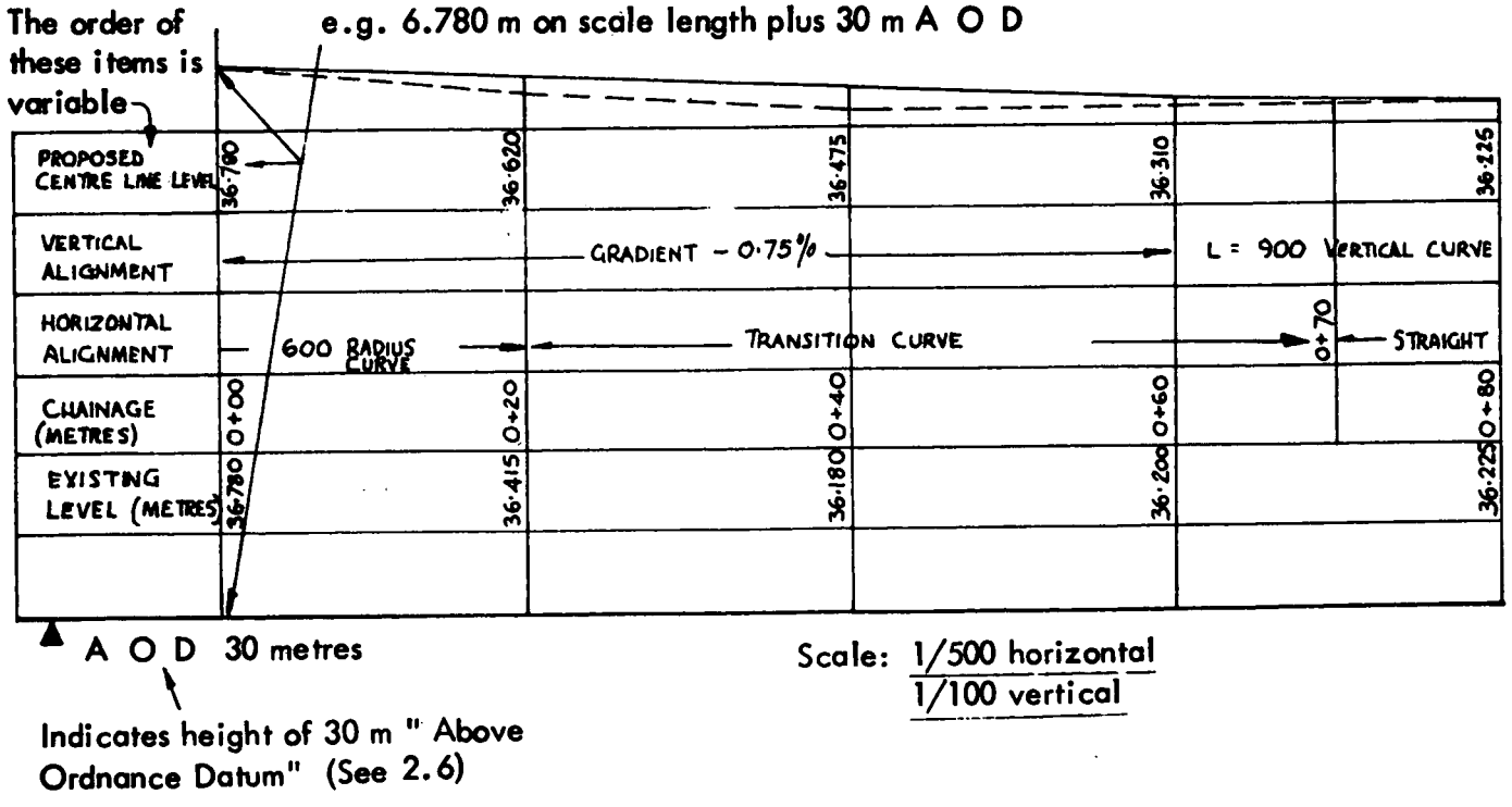
Figure 2.2 Longitudinal section along line AB in Figure 2.1 above
