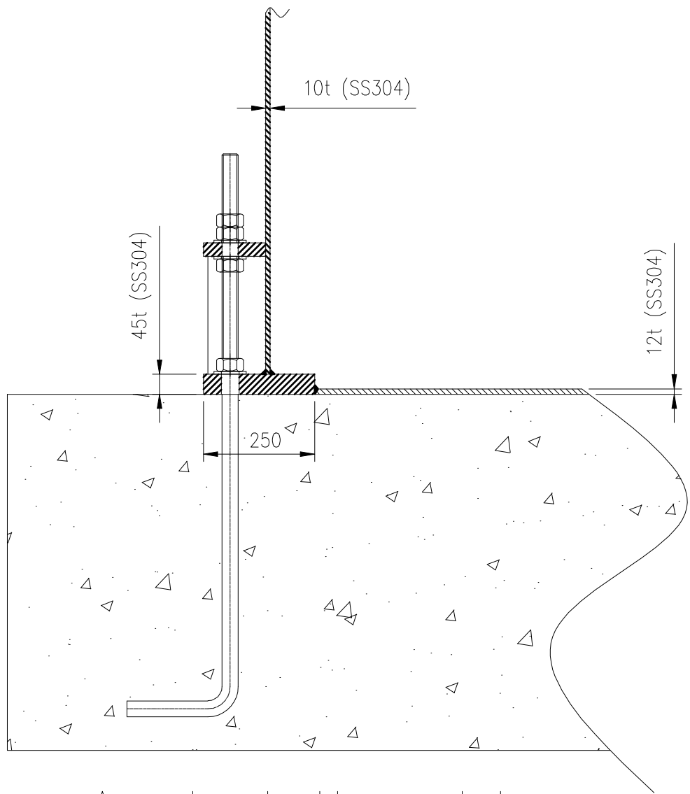
Annular bottom plate
