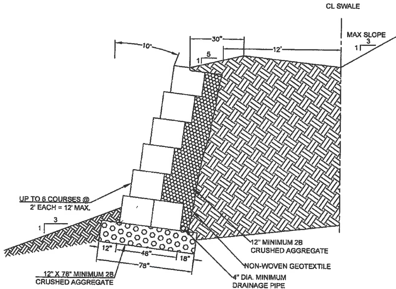
10-12 FOOT RETAINING WALL TYPICAL SECTION
