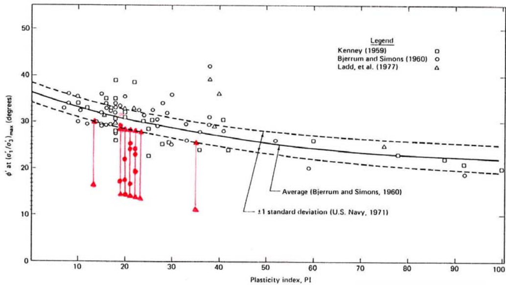
Fig. 10 – Range of residual shear strengths from actual tests on materials sampled in the Pliocene-age Orinda formation in the Mission Peak Landslide. The lower thresholds are attributable to presence of smectite clays.
