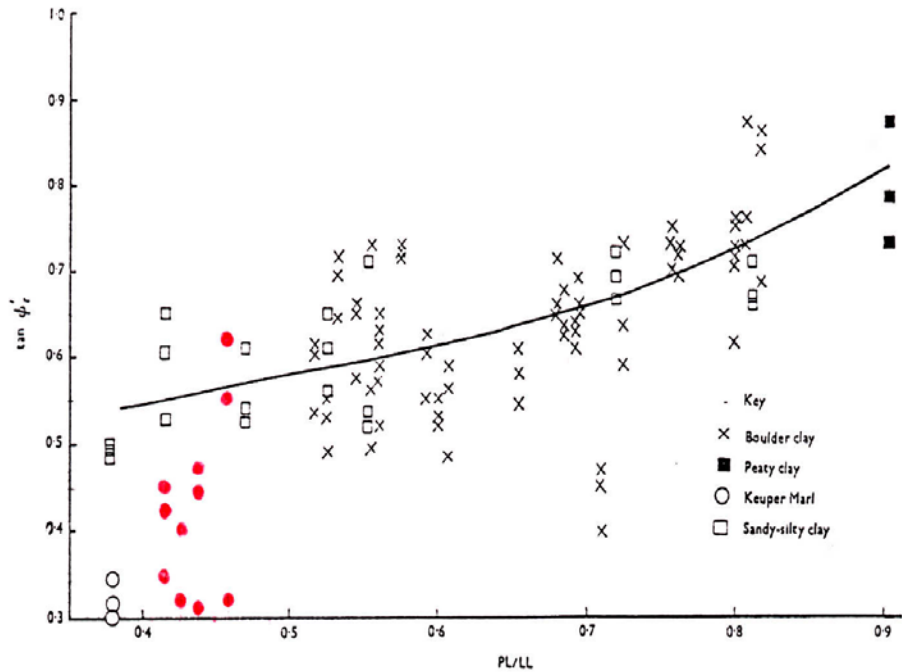
Fig. 11 — Range of residual shear strengths from actual tests on materials sampled in the Pliocene-age Orinda formation in the Mission Peak Landslide. The lower thresholds are attributable to presence of smectite clays.
