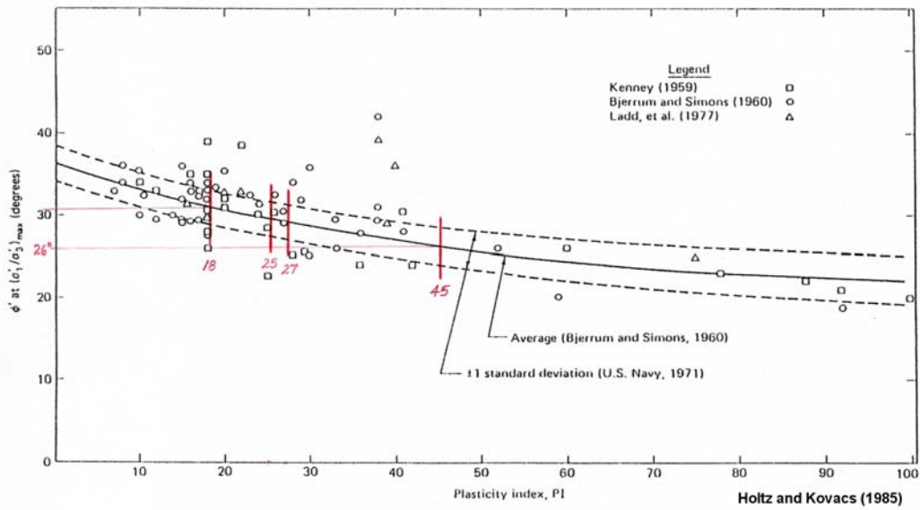
Figure 5 – Plasticity data for residual soils and landslides developed on the Rincon Shale plotted in red on a chart comparing PI with residual angle of internal friction, \phi_r , taken from Holtz and Kovacs (1985). In this plot the median values range between \phi_r = 26 and 31 degrees, which appear somewhat higher than might explain the observed sliding on this site.
