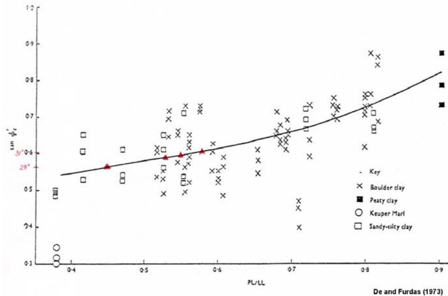
Figure 7 – Plasticity data for residual soils and landslides developed on the Rincon Shale plotted in red on a chart comparing PlasticLimit/Liquid Limit with residual angle of internal friction, \phi_r , taken from De and Furdas (1973). This plot came from data on small to medium scale slumps developed in highly overconsolidated shales in South Wales, Great Britain. In this plot the data scatter is quite large, but the median values vary between \phi_r = 29 and 31 degrees.
