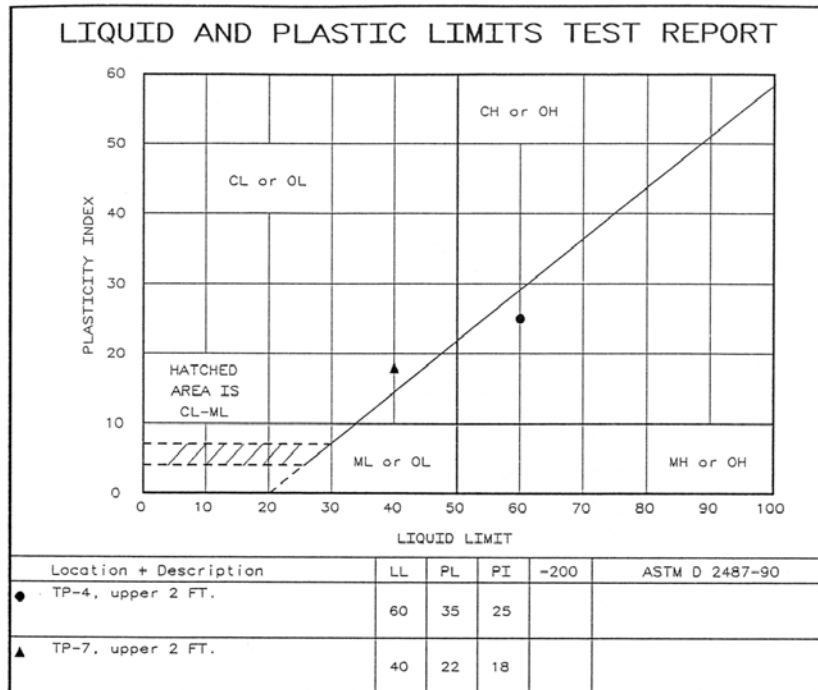
Figure 3 – Atterberg Limits test data for soil samples recovered from exploratory trenches on the subject parcel, a few hundred feet uphill of the Old Earth and Debris Flow Fan. These samples were representative of residual soils developed on the Rincon Shale.
