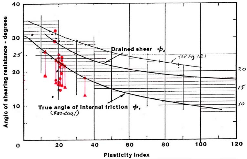
Fig. 9 – Range of residual shear strengths from actual tests on materials sampled in the Pliocene-age Orinda formation in the Mission Peak Landslide. The lower thresholds are attributable to presence of smectite clays.
