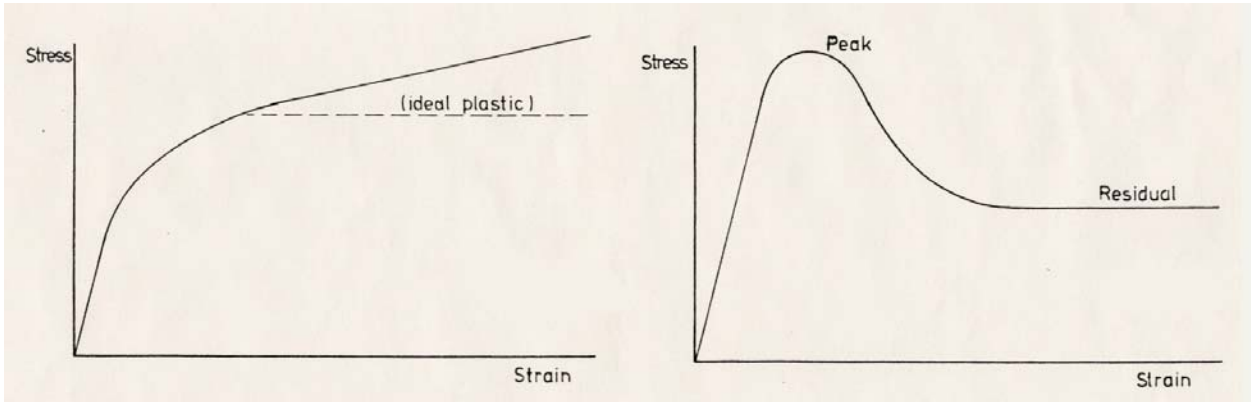
Fig. 1 presents the stress-strain behavior of two varying geologic materials involved in landslipping. The left diagram presents stress-strain behavior of a quasi-plastic, or strain-hardening material , such as normally consolidated clay. The right-hand plot shows the behavior exhibited by brittle materials, such as overconsolidated clay or bedrock, which tend to exhibit strain-softening behavior .
