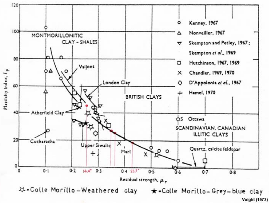
Figure 6 – Plasticity data for residual soils and landslides developed on the Rincon Shale plotted in red on a chart comparing Plasticity Index with residual angle of internal friction, \phi_r , taken from Voight (1973). This plot is comprised of residual strength data from large landslides in Montmorillonitic clay shales. The median values range between \phi_r = 14.4 and 23.2 degrees.
