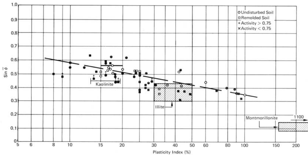
Figure 8 – Relationship between \sin \phi' and plasticity index for normally consolidated soils, using data from Kenney (1959) and Olson (1974). Note how montmorillonitic clay plots off the chart to the right.
