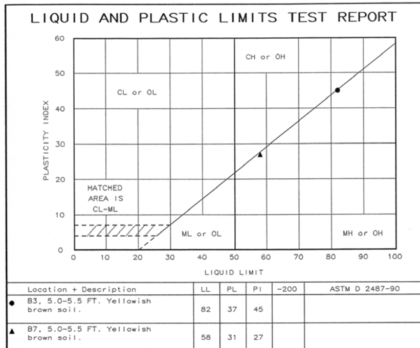
Figure 2 – Atterberg Limits test data for soil samples recovered from exploratory borings on the subject parcel, a few hundred feet uphill of the Old Earth and Debris Flow Fan. Sample B3 came from a deep-seated slump-earthflow landslide.
