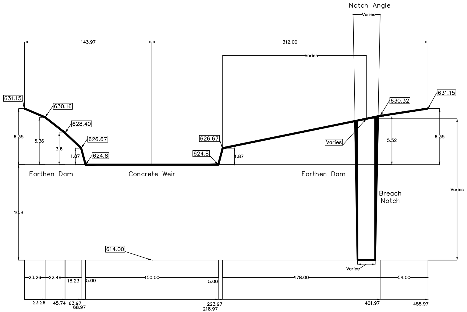
Stone Lake Dam (Vertical exaggeration= 10)
