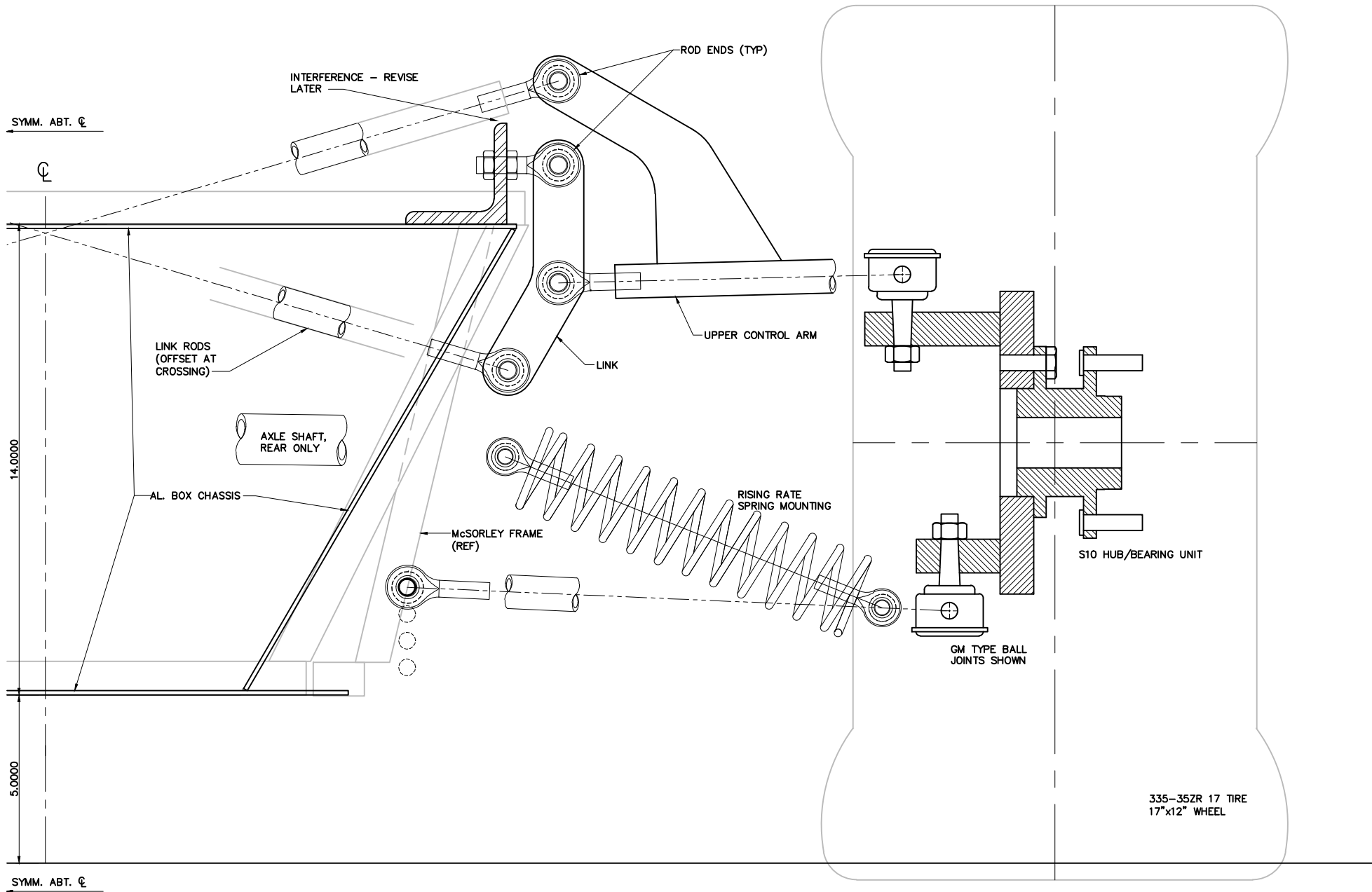
CAMBER COMPENSATING ANTI-ROLL SUSPENSION SCALE: 3" = 1'-0"
