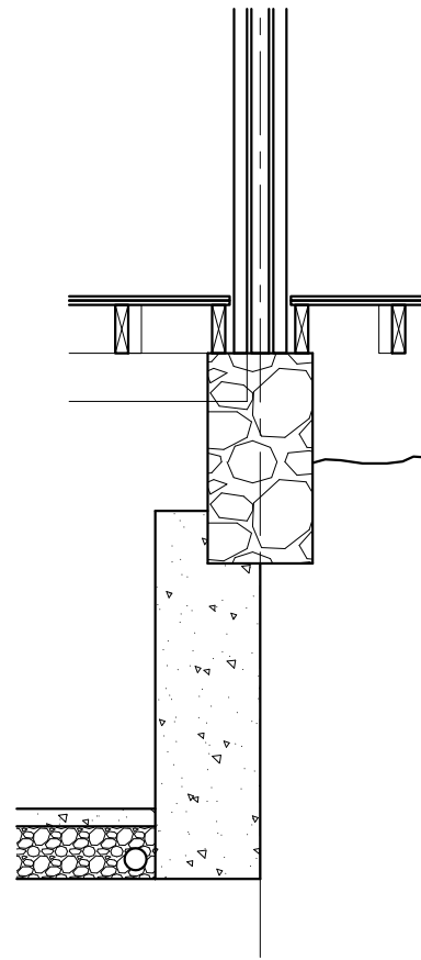
OPTION B
