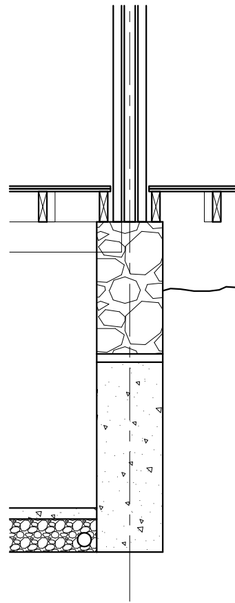
OPTION A
