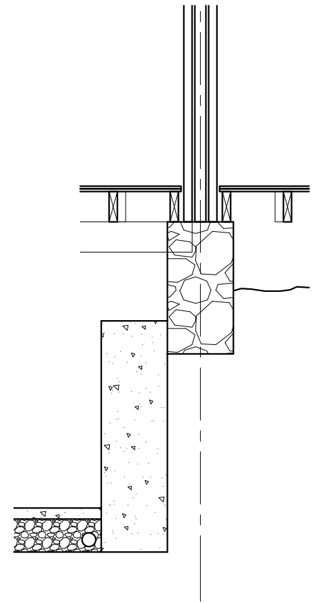
OPTION C
