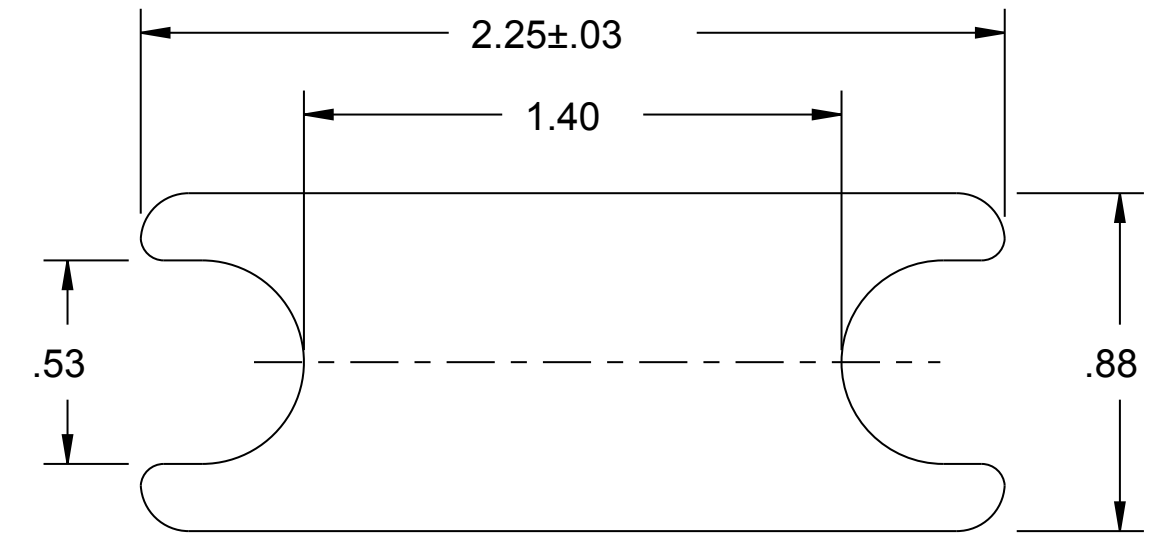
FLATTENED VIEW SCALE: 2/1
