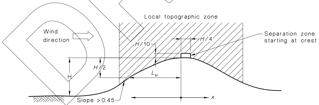
FIGURE 4.4 SEPARATION ZONE FOR HILLS AND ESCARPMENTS HAVING UPWIND SLOPES GREATER THAN 0.45
