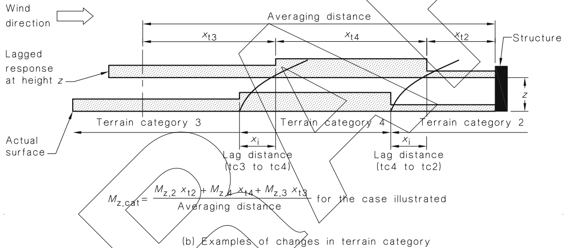
FIGURE 4.1 CHANGES IN TERRAIN CATEGORY
