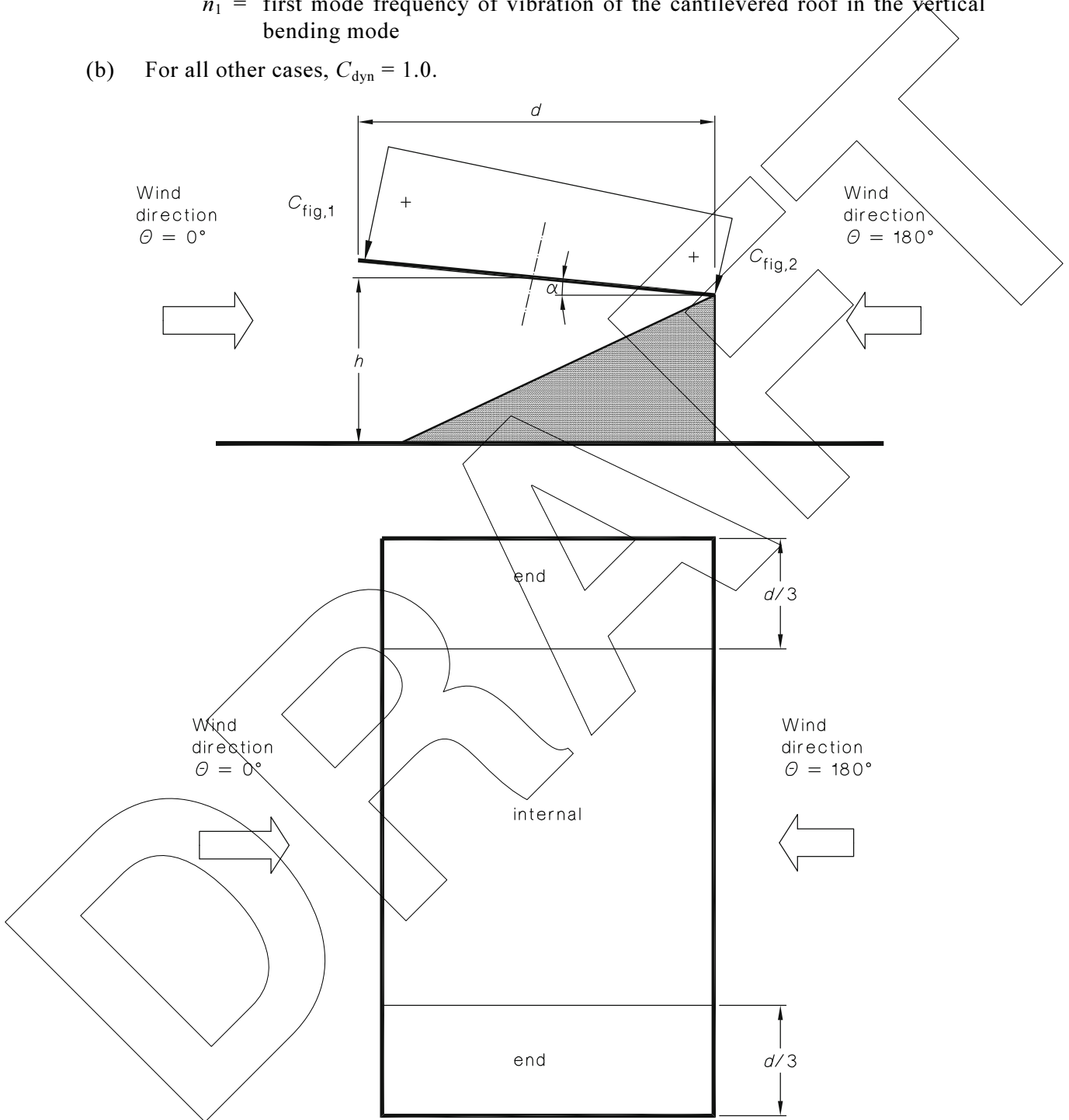
FIGURE D7 CANTILEVERED ROOF
