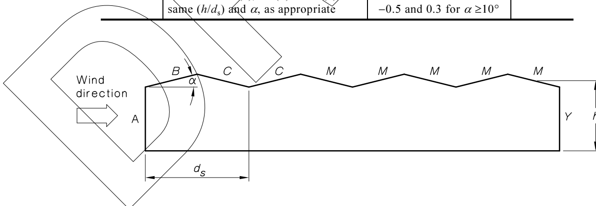
FIGURE C1 EXTERNAL PRESSURE COEFFICIENTS ( C_{p,e} ) FOR MULTI-SPAN BUILDINGS—PITCHED ROOFS
