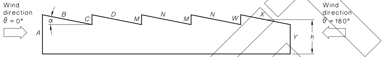
FIGURE C2 EXTERNAL PRESSURE COEFFICIENTS ( C_{p,e} ) FOR MULTI-SPAN BUILDINGS—SAW-TOOTH ROOFS
