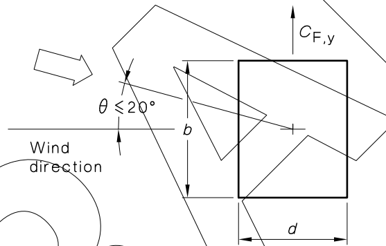
FIGURE E2(A) ALONG-WIND COEFFICIENTS FOR RECTANGULAR PRISMS
