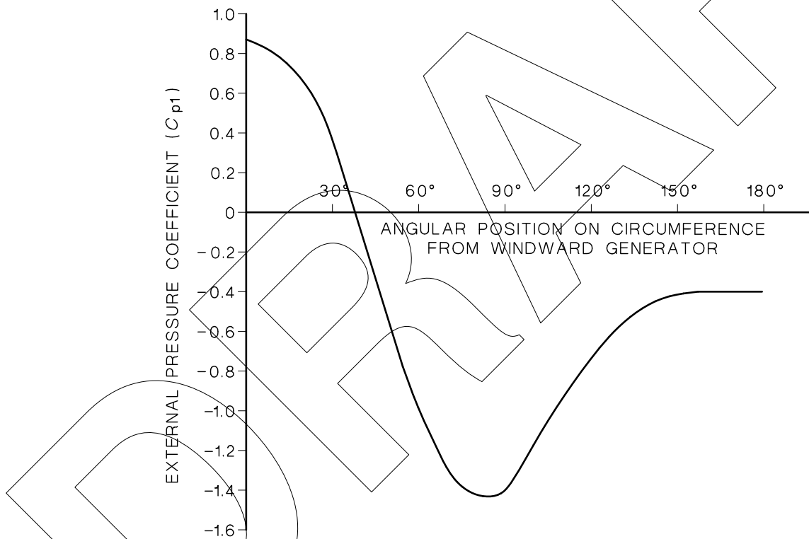
FIGURE C6 PLOT OF EXTERNAL PRESSURE COEFFICIENTS ( C_{p1} ) ON WALLS OF CIRCULAR BINS, SILOS AND TANKS ( c/b = 1 )
