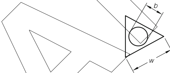
(f) Cylindrical ancillary inside triangular tower
