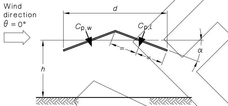
FIGURE D3 PITCHED FREE ROOFS
