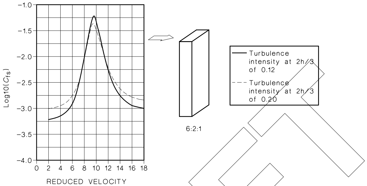
FIGURE 6.4 CROSSWIND FORCE SPECTRUM COEFFICIENT FOR A 6:2:1 RECTANGULAR SECTION
