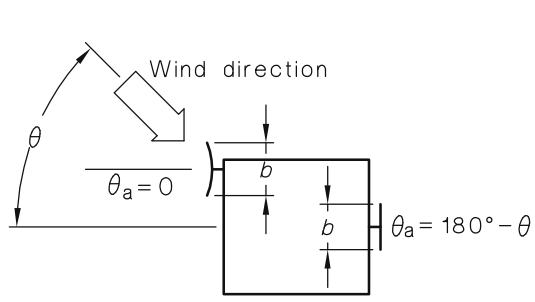
(a) Ancillary attached to face of square tower
