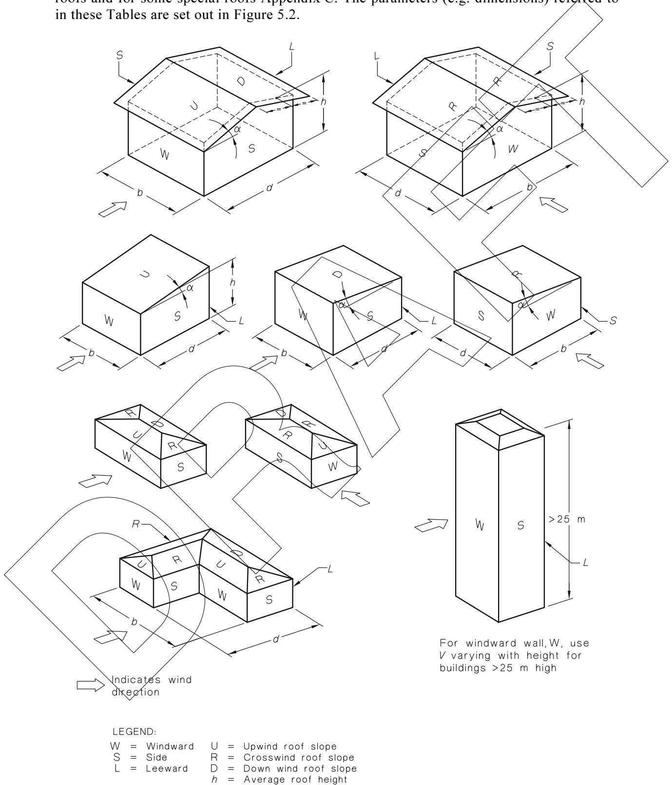
FIGURE 5.2 PARAMETERS FOR RECTANGULAR ENCLOSED BUILDINGS
