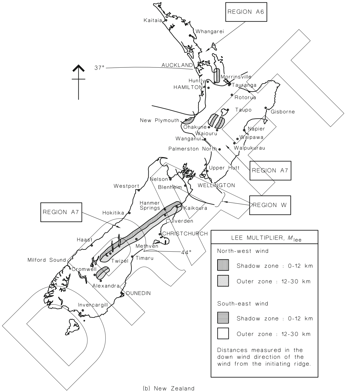
FIGURE 3.1(B) WIND REGIONS
