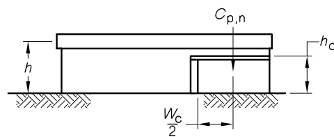
(c) Wall on two sides
