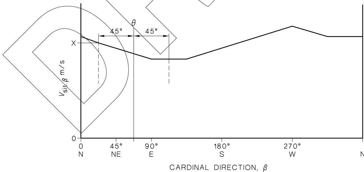
FIGURE 2.2 RELATIONSHIP OF WIND DIRECTIONS AND BUILDING ORTHOGONAL AXES
