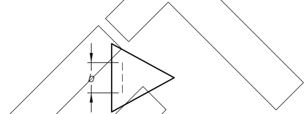
(b) Ancillary attached to face of triangular tower
