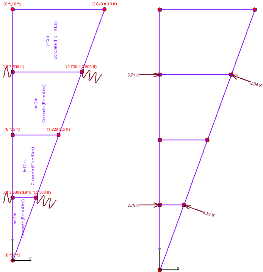
Case 1 – 12" Concrete Plate Element
