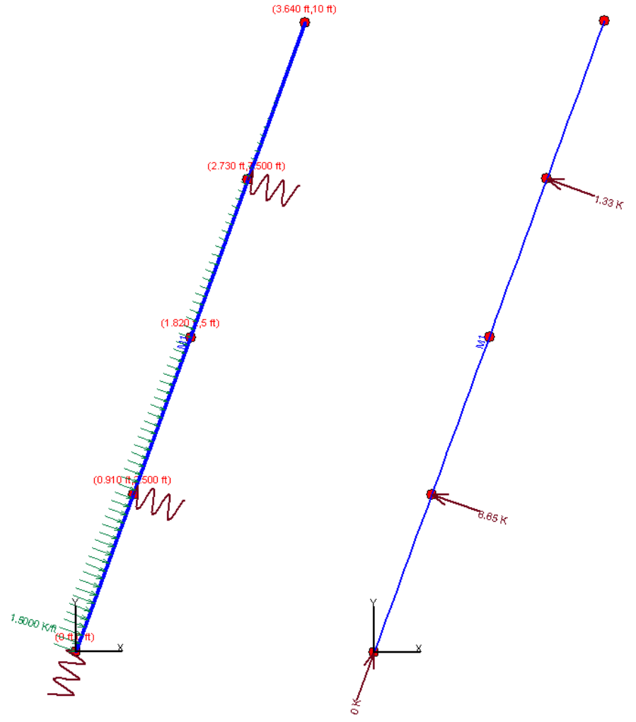
Case 2 – Linearly Distributed Load – Placed Normal to beam
