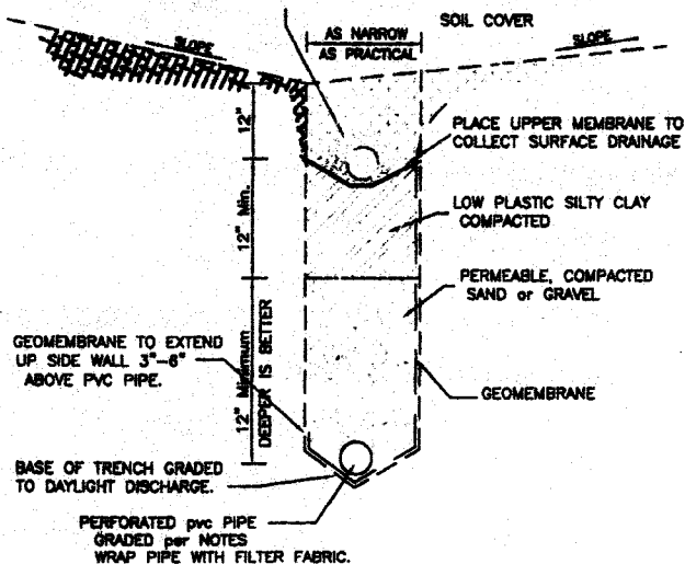
SHALLOW MOISTURE BARRIER & AREA DRAINS BETWEEN STRUCTURES OR BELOW HILLSIDE. CLEAN SAND or CLEAN GRAVEL OPTION
