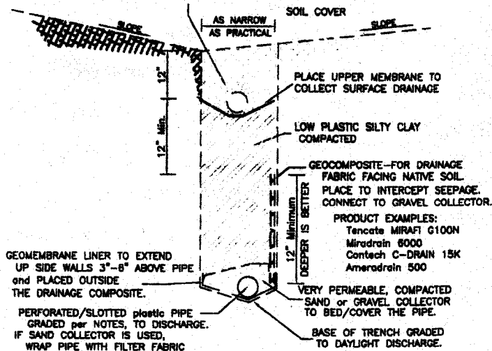
SHALLOW MOISTURE BARRIER & AREA DRAINS BETWEEN STRUCTURES OR BELOW HILLSIDE. GEOCOMPOSITE DRAIN OPTION
