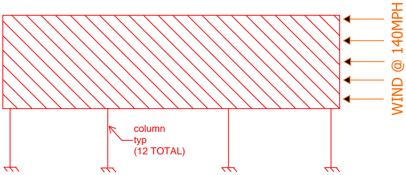
SIDE ELEVATION VIEW (SECTION A-A)
