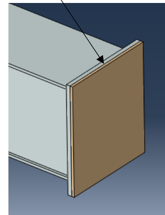
Bolted Flanges sealed by O-rings
