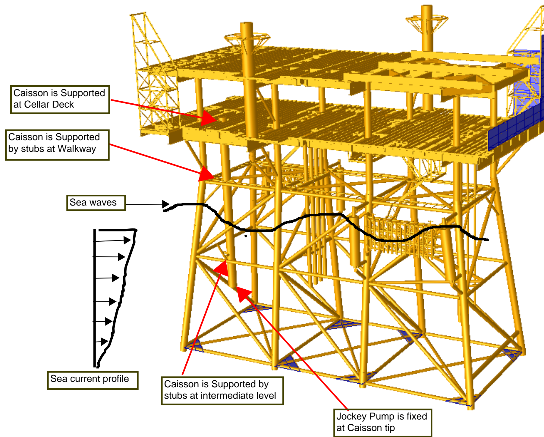
An illustration for environmental loading acting on the platform and Caisson supporting conditions
