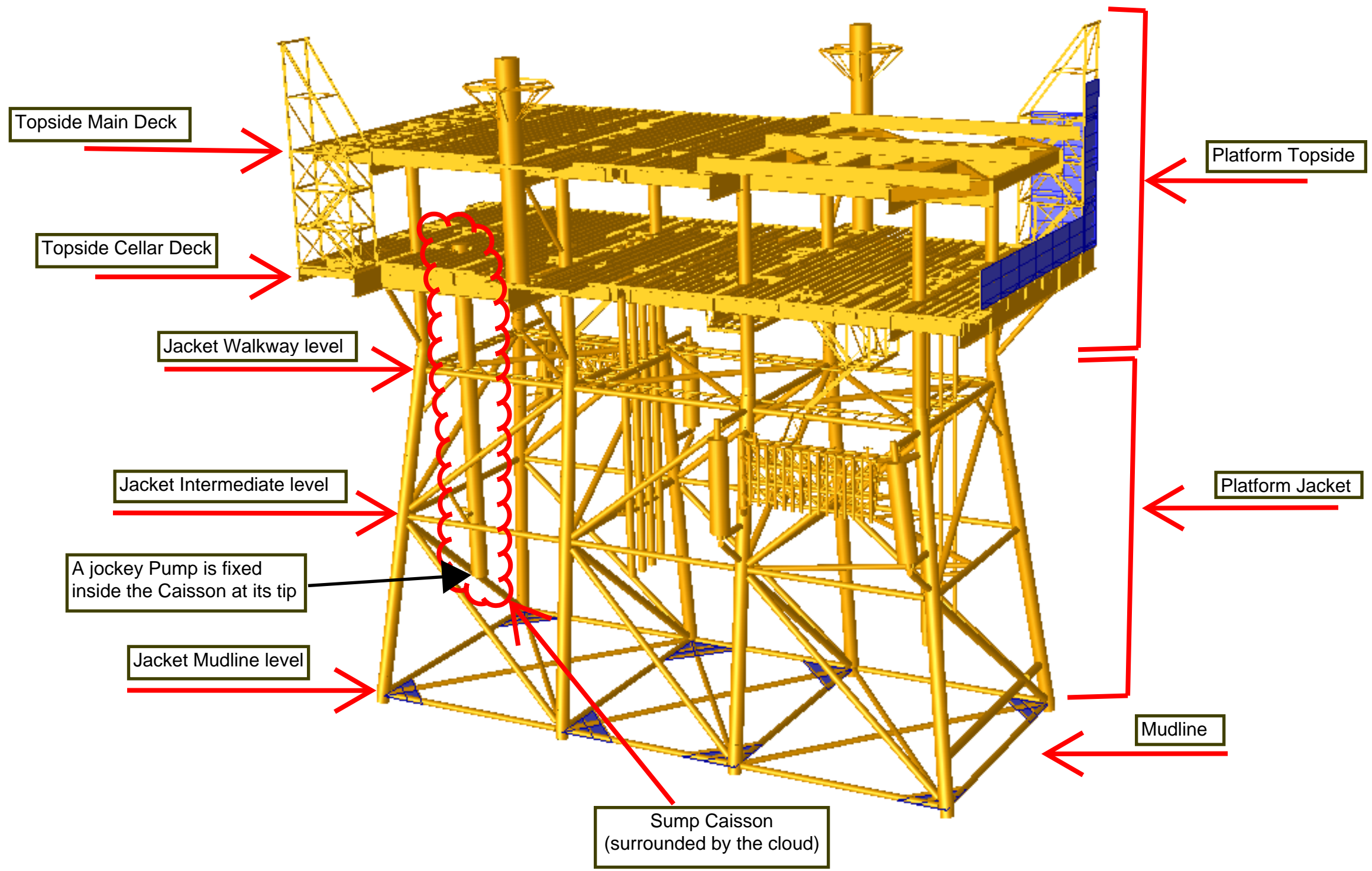
Platform description and an illustration for the Sump Caisson location
