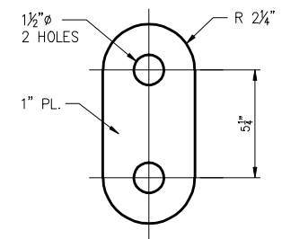
LINK - MK L1 4 REQ'D
