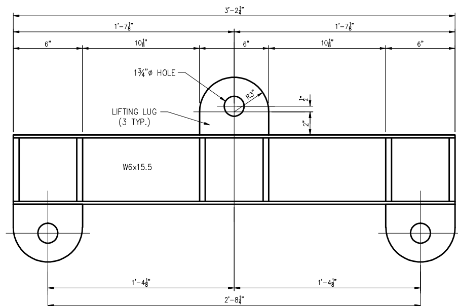
BEAM - MK B1 ONE REQ'D
