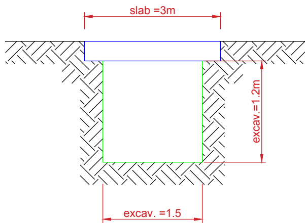
SECTION A-A AFTER EXCAVATION
