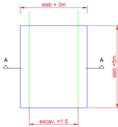
PLAN VIEW
