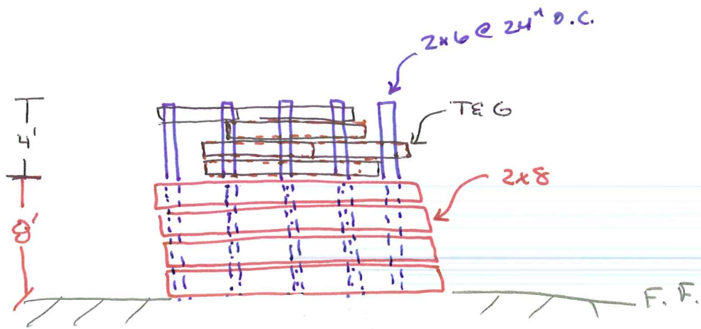
Elev. View
