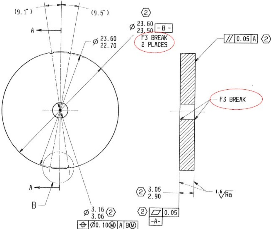
SECTION A/A
