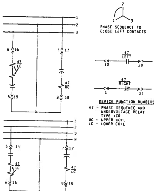
Figure 5 (0376A0953-3) Typical External Connections for Type ICR53B Relay
