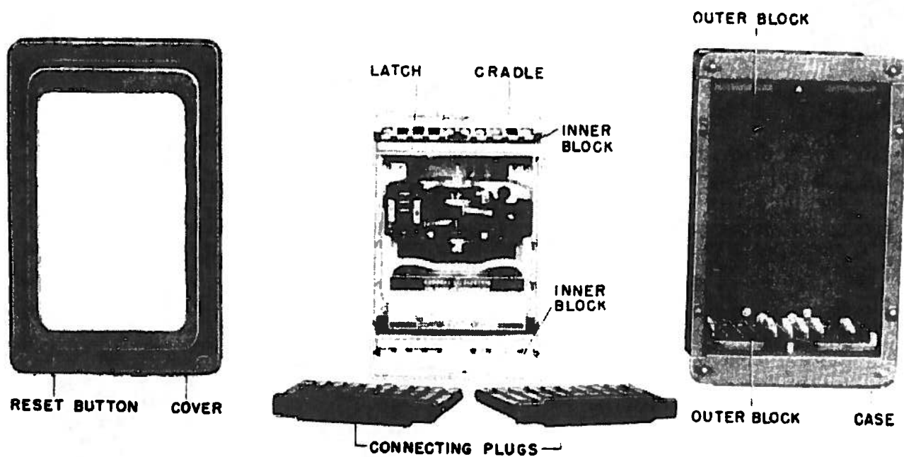
Figure 1 (8014332) Type ICR53A Relay, Unit Disassembled (Front View)
