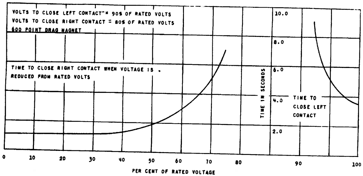
Figure 2B (0376A0950) Average Time Characteristic of Relay Types ICR53A and ICR53B
