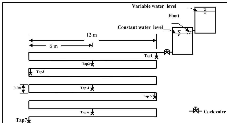
Fig. (2) Schematic diagram of pilot distribution system
