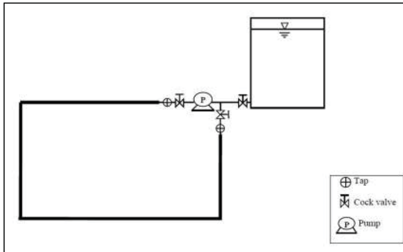
Fig. (4) Schematic diagram of pilot Loop system
