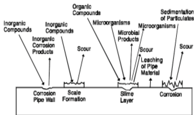
Fig. (1) Schematic of chemical and microbiological transformation at the pipe wall [3]
