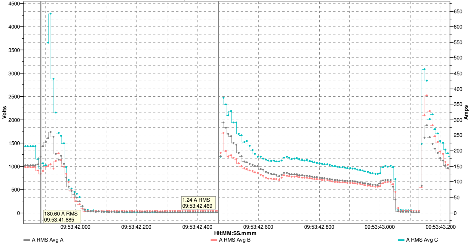
Figure 2 –Current Trend at time of interruption
