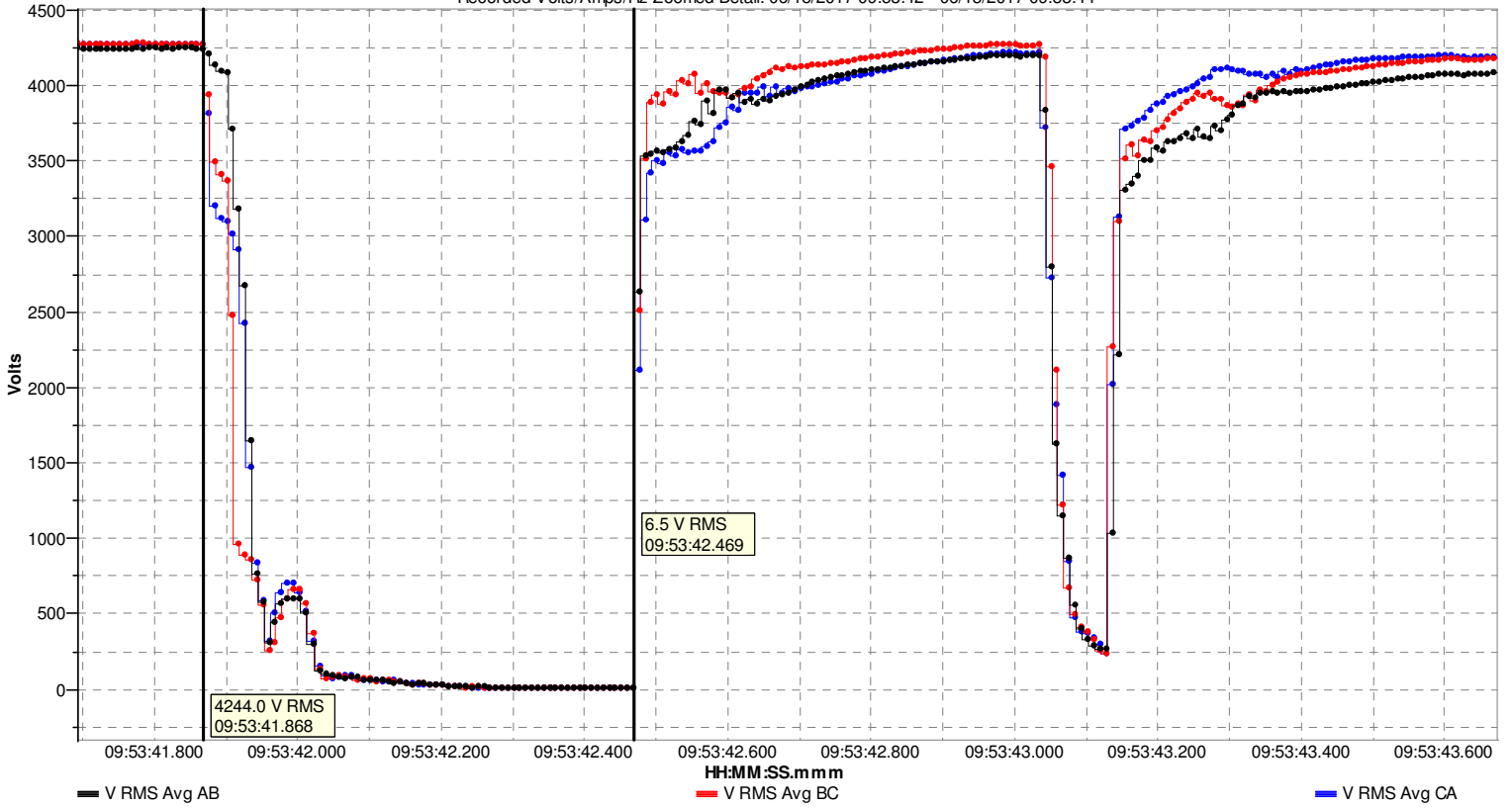
Figure 1 – Voltage Trend at time of interruption
