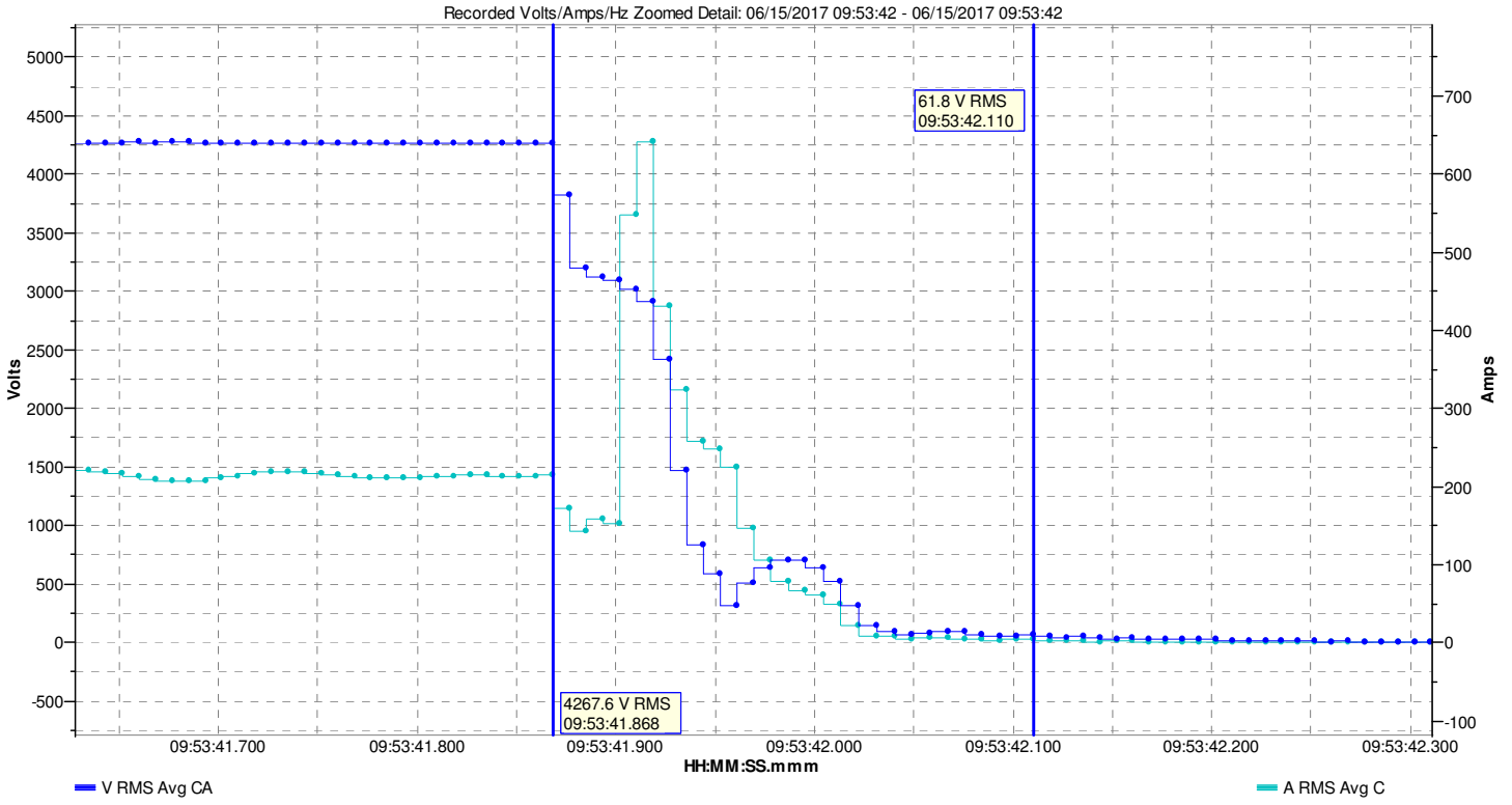
Figure 3 –Voltage and current trend on one phase during time of interruption
