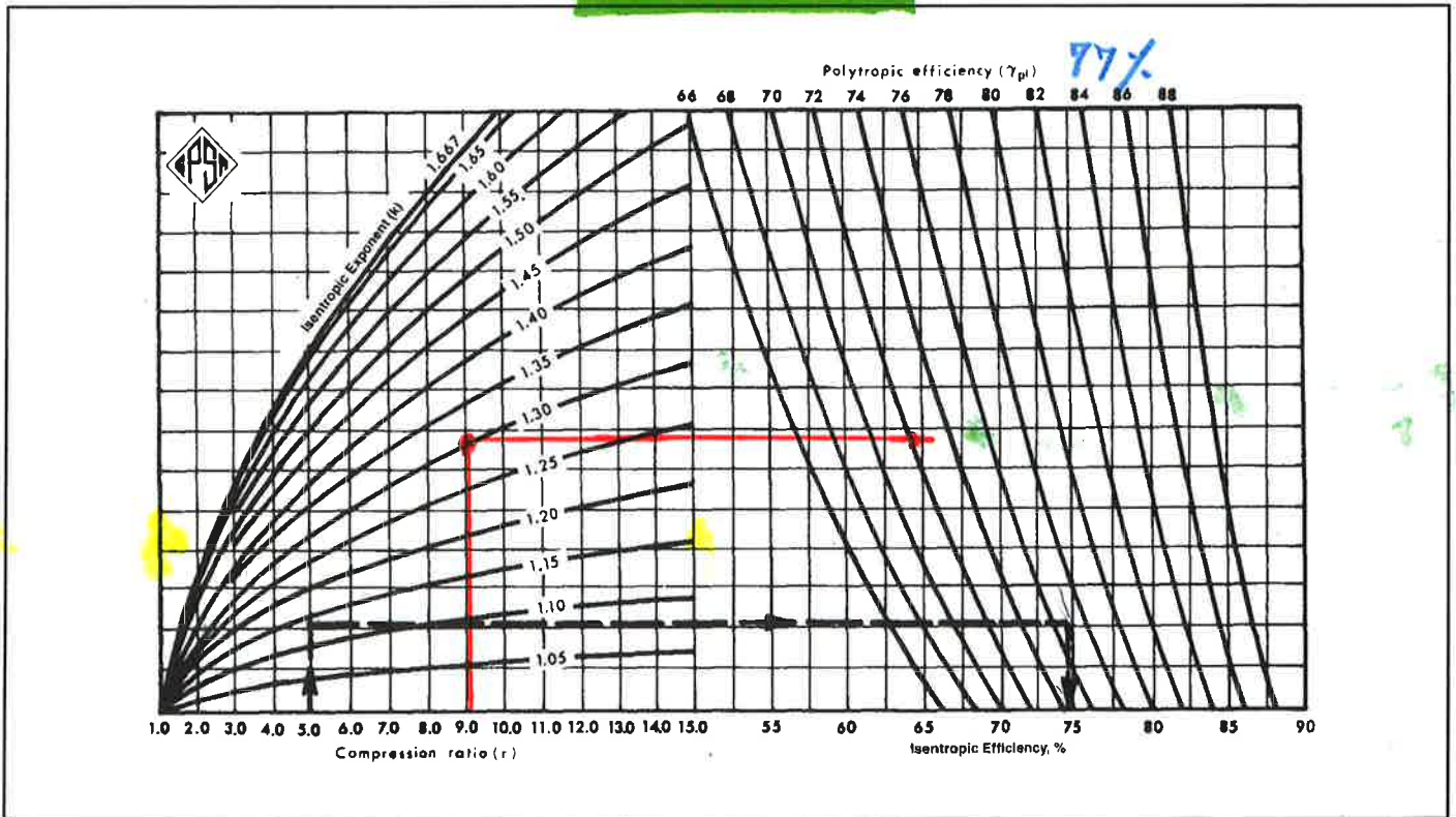
FIG. 13-35 Efficiency Conversion
