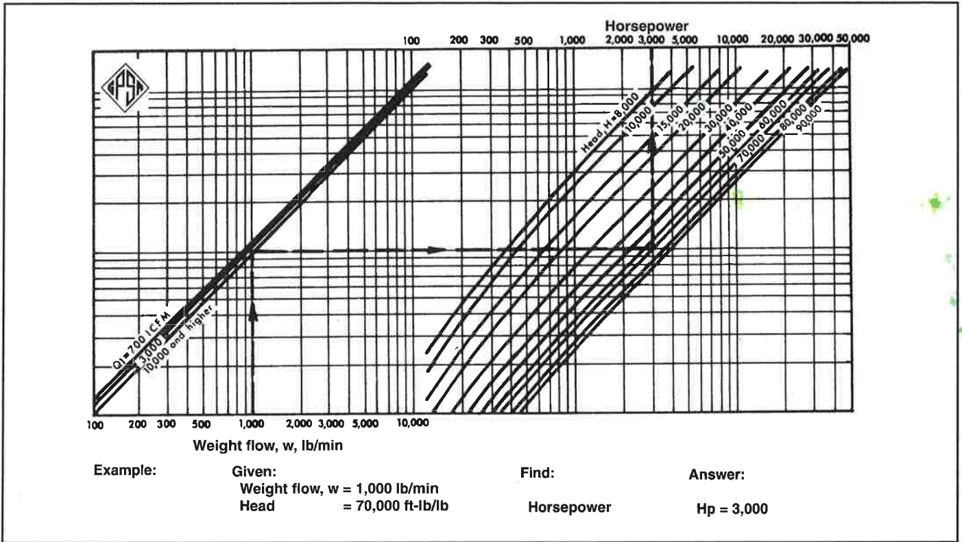
FIG. 13-34 Horsepower Determination
