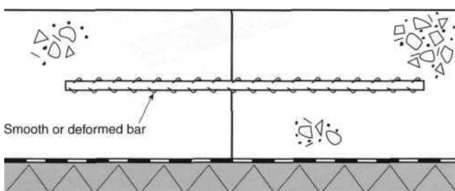
Figure 8.4: Formed restrained-movement joint
