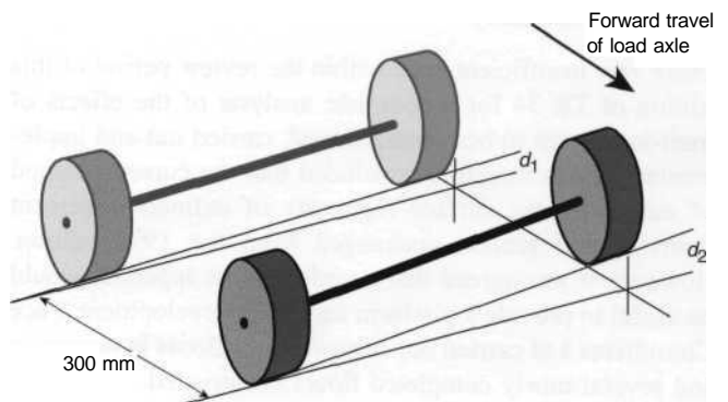
Figure C3: Property B ( = d_2 - d_1 )
