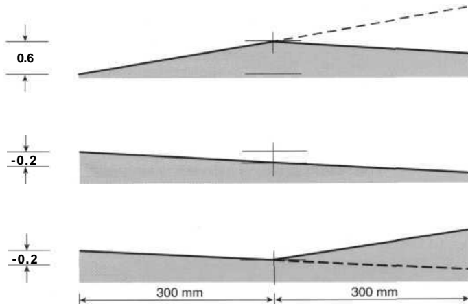
Figure 4.3: Examples of measurements of Property I over 300 mm and the resultant determination of change in elevational difference over a distance of 300 mm (Property II). All dimensions in mm.
