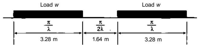
Figure B3: Arrangement of loads for maximum hogging moment
