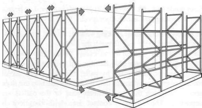
Figure 3.5: Mobile pallet racking.
