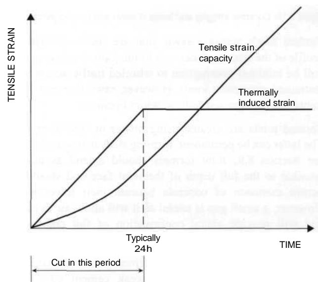
Figure 8.9: Suggested mechanism of crack induction.
