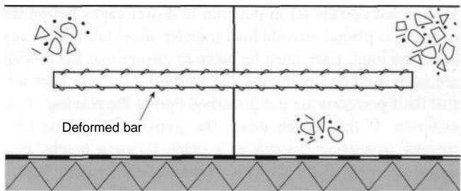
Figure 8.5: Tied joint
