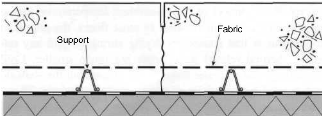
Figure 8.3: Sawn restrained-movement joint (shown with fabric).
