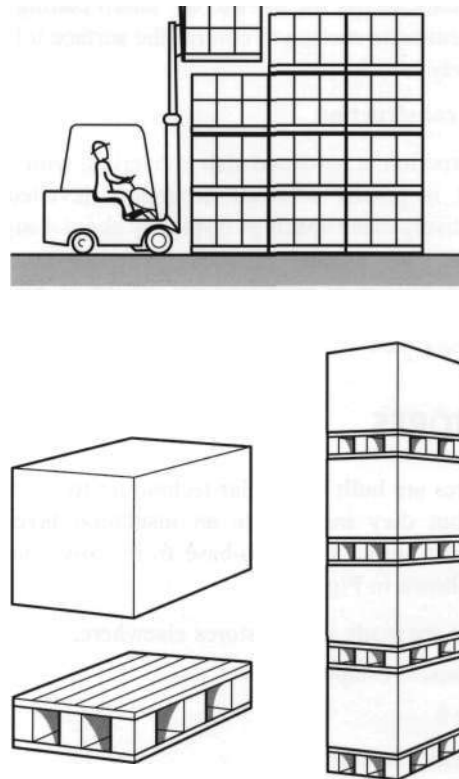
Figure 3.1: Block stacking of unit loads.
