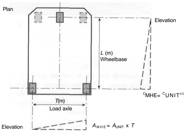
(a) Schematic of MHE.
