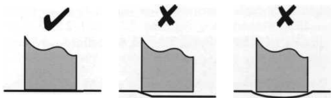
Figure 4.9: Remediation in wheel tracks.
