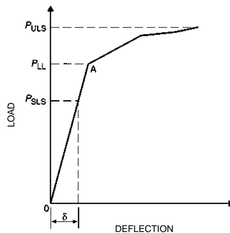
Figure 9.12: Typical load-deflection relationship for steel-fibre-reinforced ground-supported slab.
