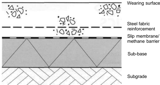
Figure 2.1: Typical slab construction.
