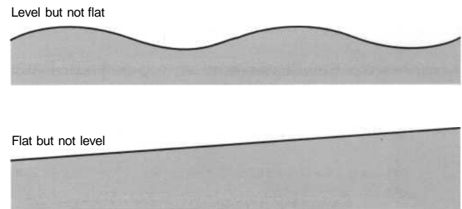
Figure 4.2: Flatness and levelness.
