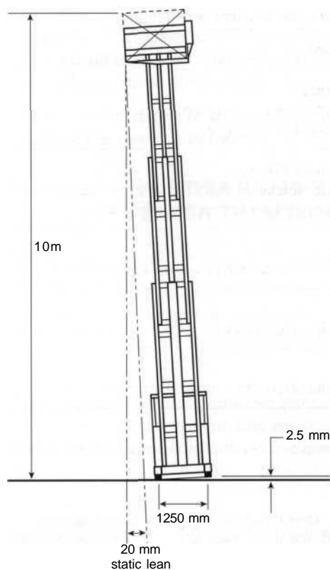
Figure 4.6: Static lean.
