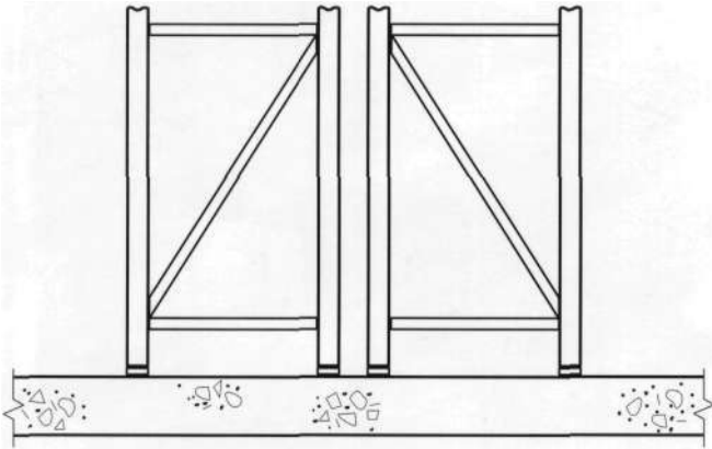
Figure 3.4: Typical 'back-to-back' configuration of storage racking.
