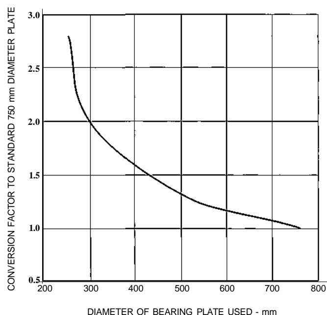
Figure 6.1: Conversion factors for different loading plate sizes.
