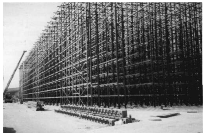
Figure 3.12: Clad rack system.
