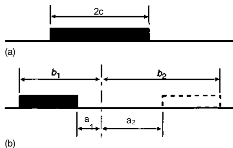
Figure 9.9: Defined areas of uniformly distributed load.
