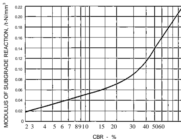
Figure 6.2: Relationship between modulus of subgrade reaction and in situ CBR.
