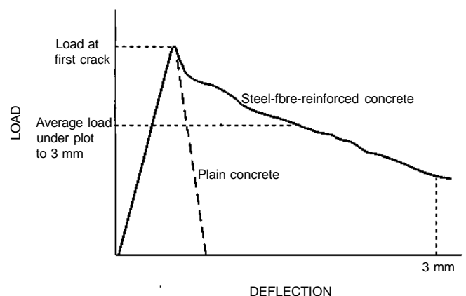
Figure 7.2: Typical load-deflection graph for steel-fibre-reinforced concrete beams.
