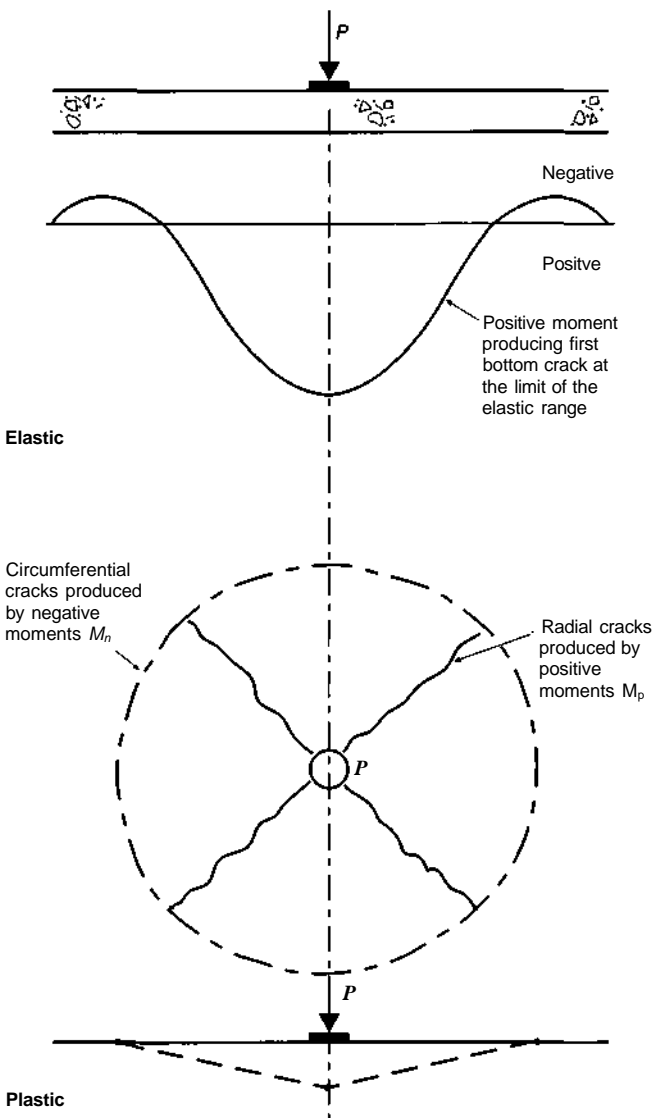
Figure 9.2: Development of radial and circumferential cracks in a concrete ground-supported slab.
