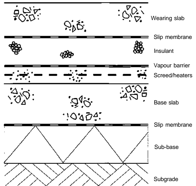
Figure 2.4: Typical construction layers in cold stores.
