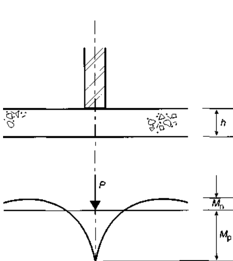
Figure 9.7: Use of Hetenyi's equations for a line load P .
