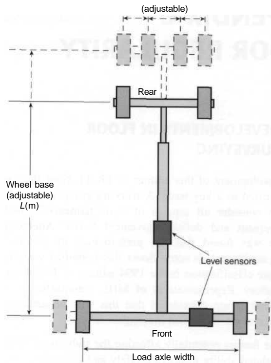
(b) Schematic of profileograph
