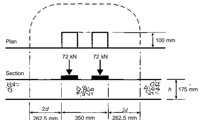
Figure B2: Punching shear perimeter at edge.
