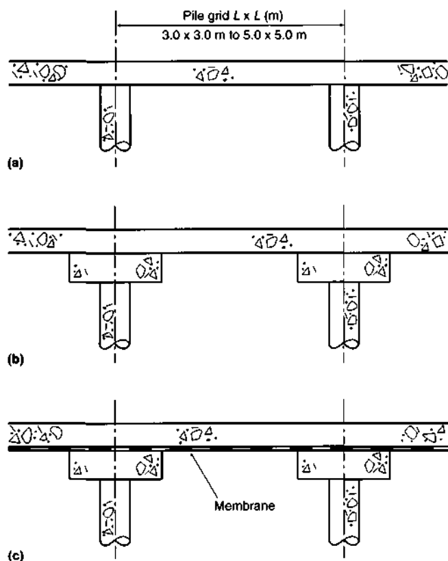
Figure D1: Cross-sections of typical piled slabs (not to scale).
