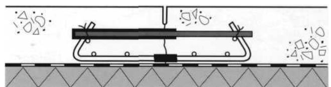
Figure 8.1: Sawn free-movement joint.
