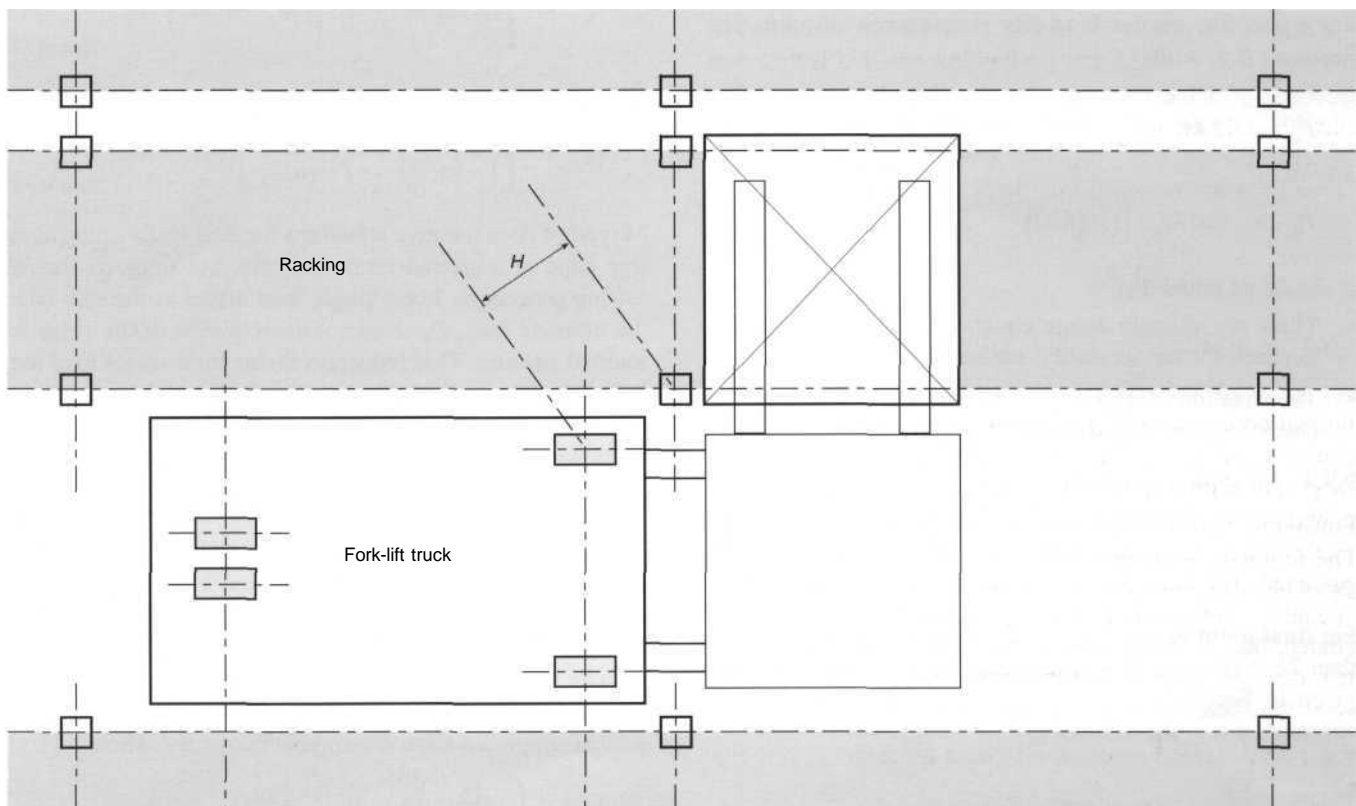
Figure 9.5: Adjacent point loads in very narrow aisles.
