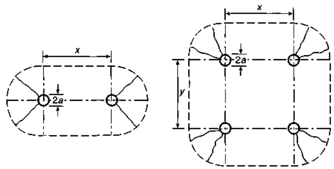
(a) Dual point loads. (b) Quadruple point loads.
