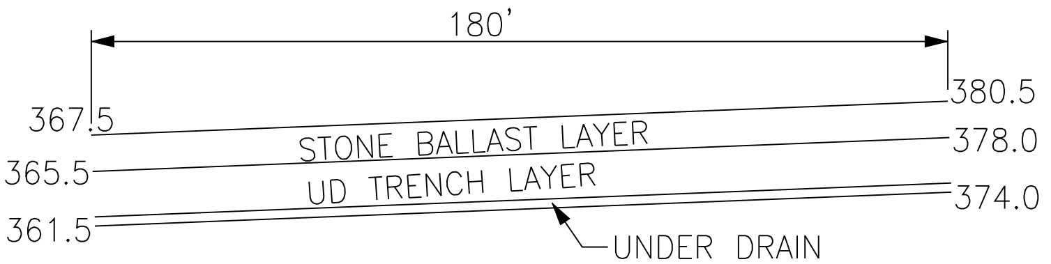
PROFILE
