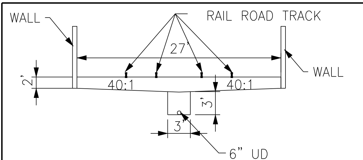
CROSS SECTION
